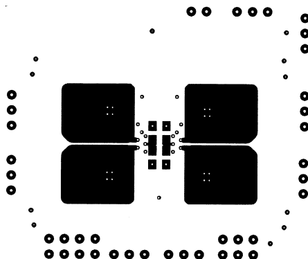
Figure 14. Recommended PC board layout: Bottom side layout
