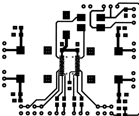
Figure 11. Recommended PC board layout: Component side layout
