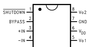
Figure 3. SOIC Package – Top View See Package Number D
