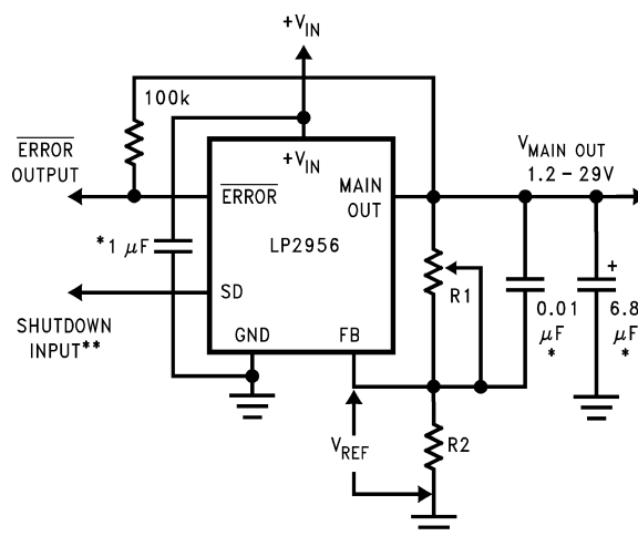
Figure 42. Adjustable Regulator
