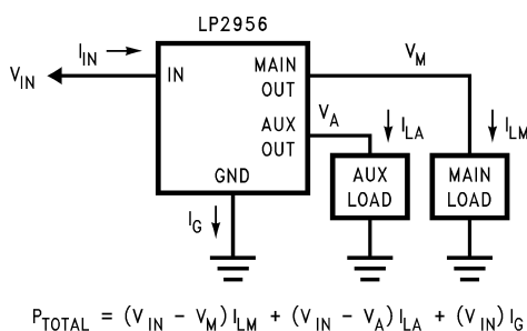
Figure 40. Current/Voltage Diagram
