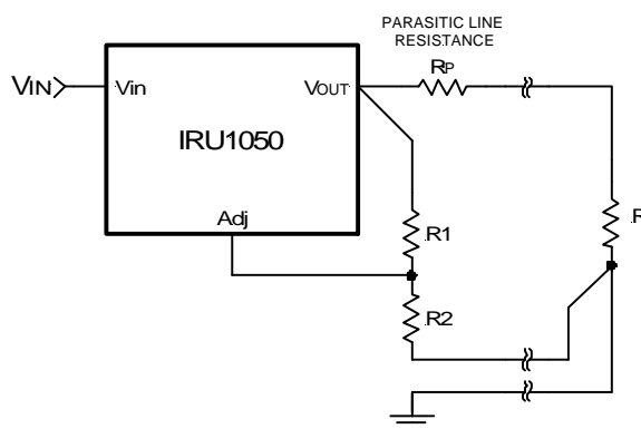
Figure 4 - Schematic showing connection for best load regulation.
