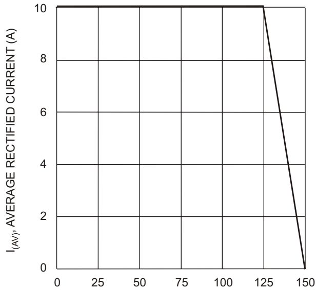
T_C , CASE TEMPERATURE ( ^{\circ}\text{C} )
