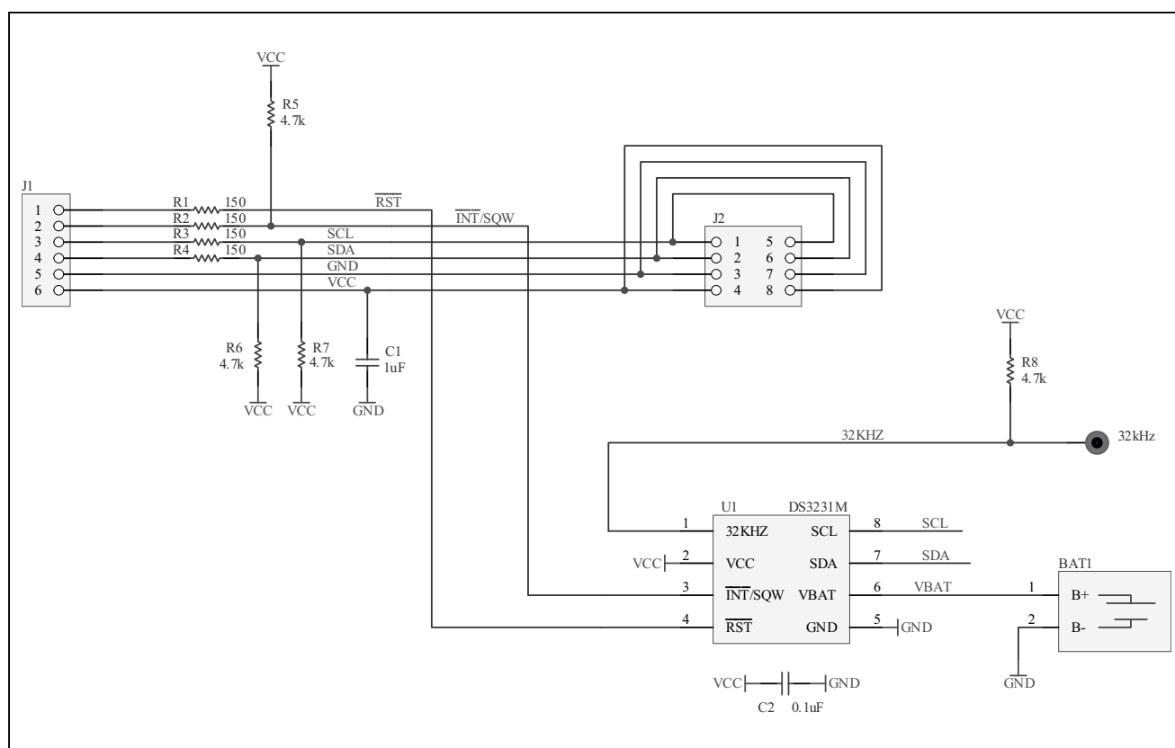
Figure 1. DS3231MPMB1 Peripheral Module Schematic
