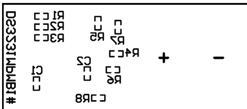
Figure 7. DS3231MPMB1 Peripheral Module Component Placement Guide—Solder Side
