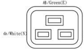
插頭端面圖 (Dimensions of Plug Face)
