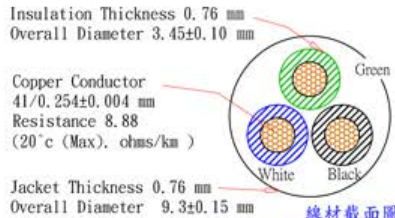
線材截面圖 (Wire Cross-Section)
