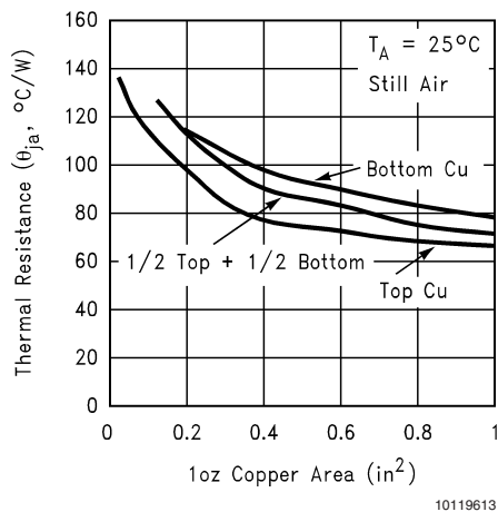
FIGURE 7. \theta_{JA} vs. 1oz Copper Area for SOT-223
