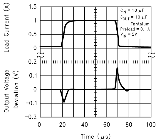
LMS8117A-3.3 Load Transient Response
