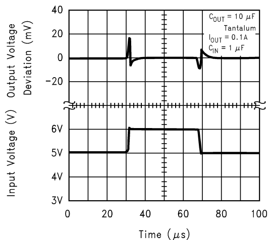
LMS8117A-3.3 Line Transient Response
