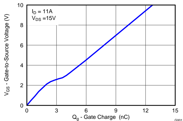
Gate Charge
