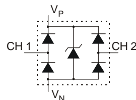
Device Schematic
