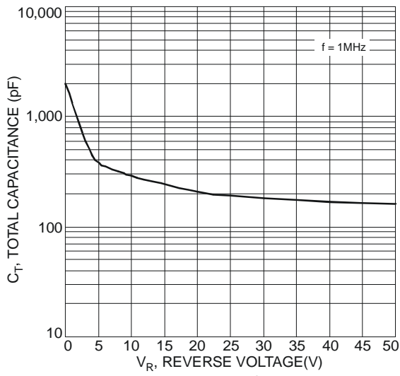
Fig 3. Typical Total Capacitance
