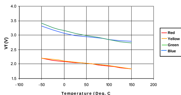
Forward Voltage vs Temperature
