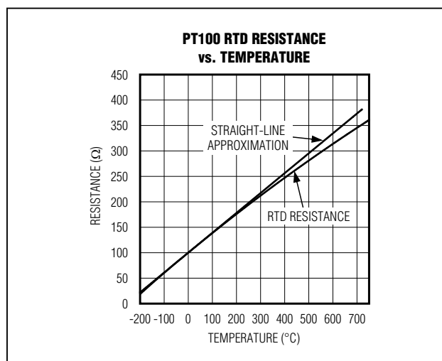
Figure 3. PT100 RTD resistance vs. temperature.
