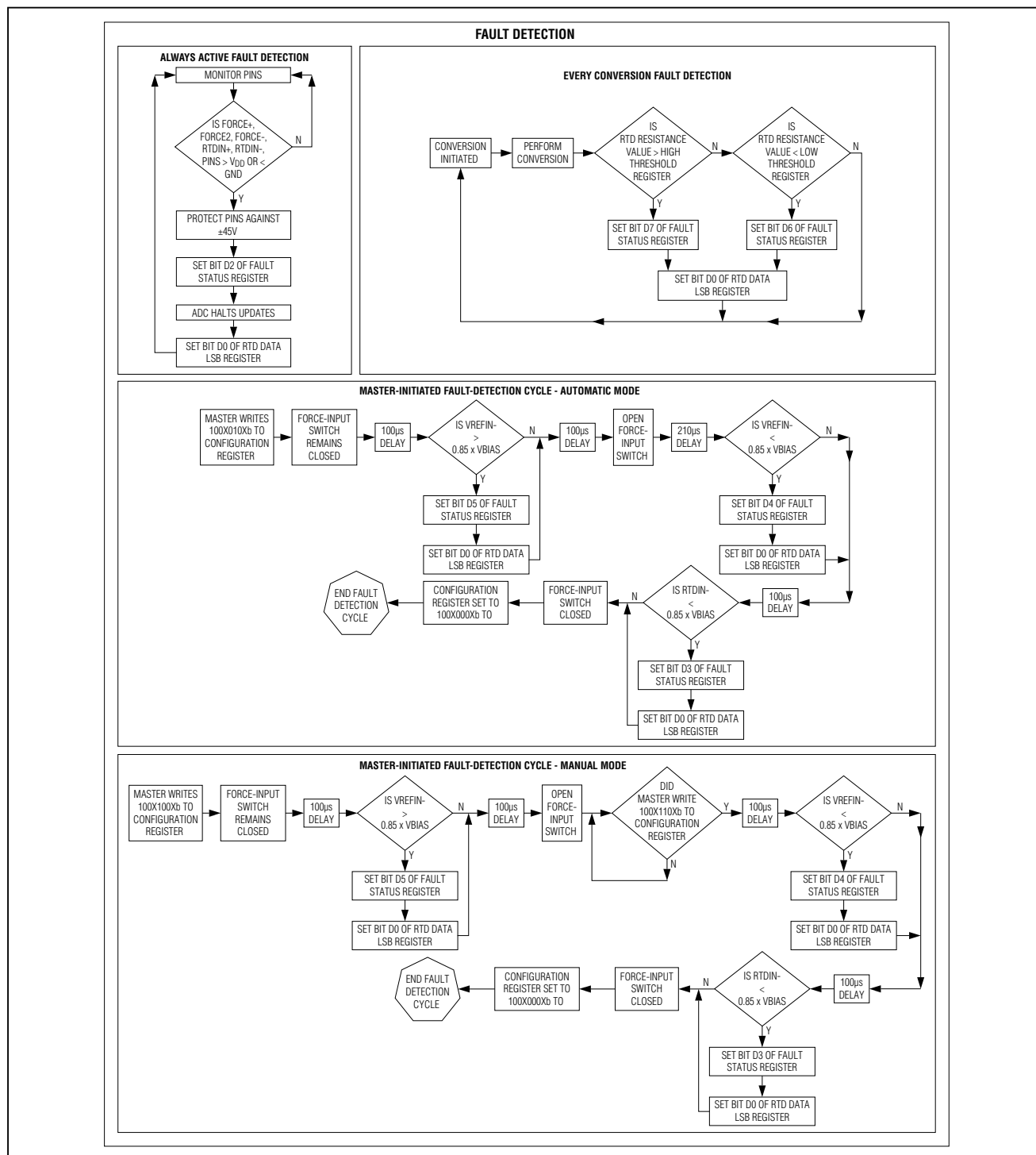
Figure 4. Fault Detection Flowcharts
