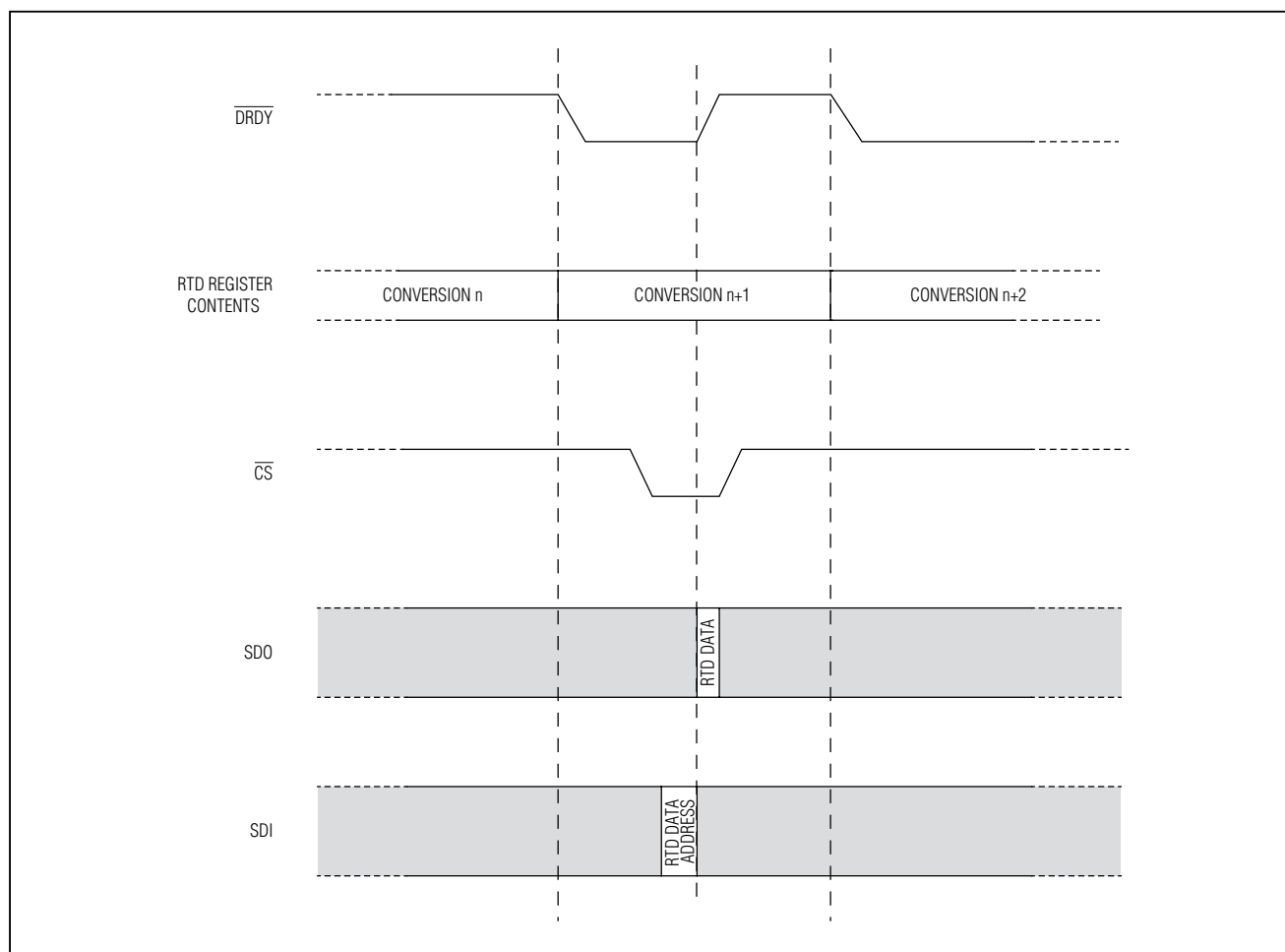
Figure 9. \overline{\text{DRDY}} Operation
