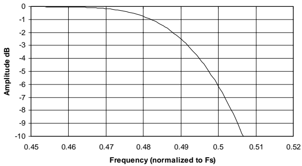
Figure 9. Single-speed Transition Band
