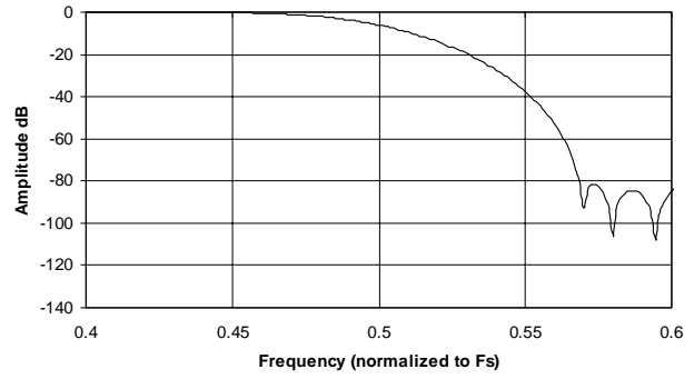
Figure 12. Double-speed Transition Band
