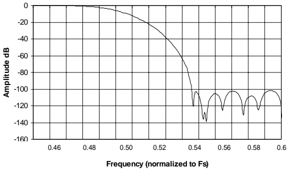
Figure 7. Single-speed Transition Band
