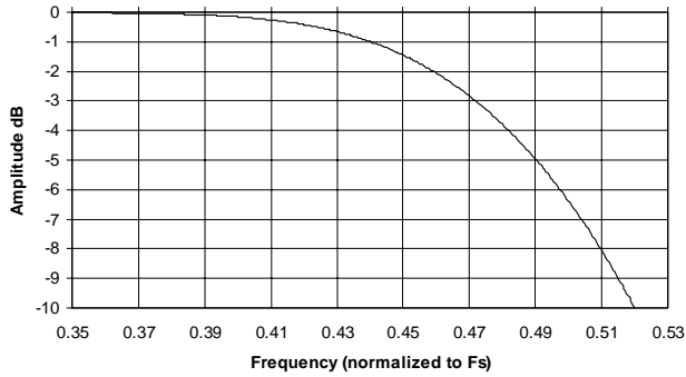
Figure 17. Quad-speed Transition Band
