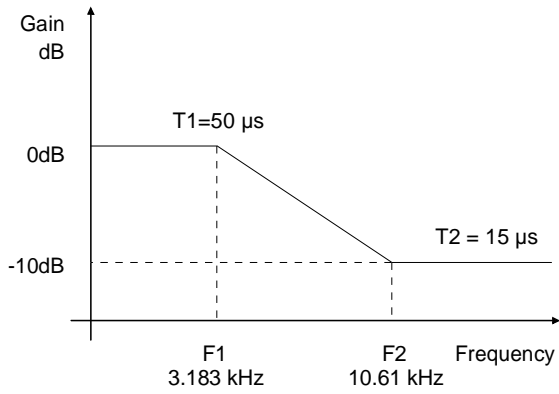
Figure 19. De-Emphasis Curve
