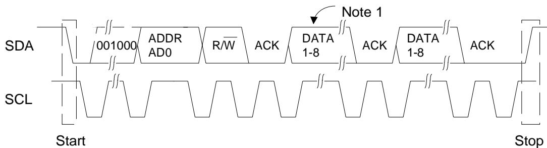
Figure 6. Control Port Timing, I 2 C Mode
