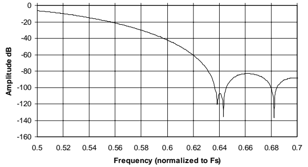
Figure 16. Quad-speed Transition Band
