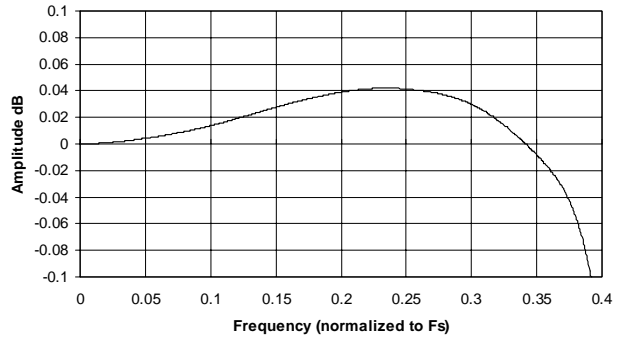
Figure 18. Quad-speed Frequency Response
