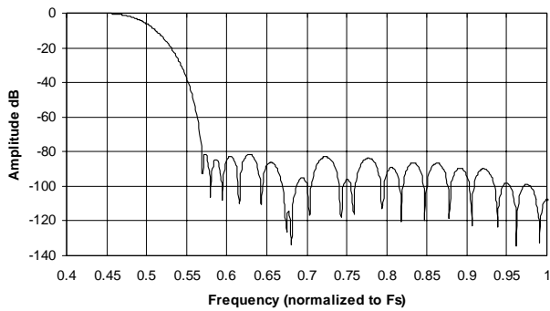
Figure 11. Double-speed Stopband
