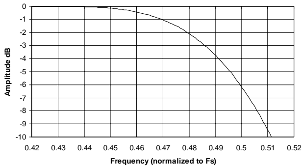
Figure 13. Double-speed Transition Band
