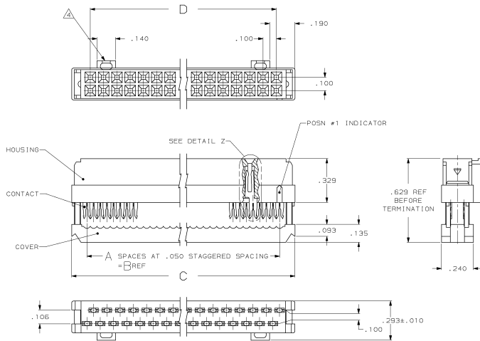
TERMINATED VIEW
