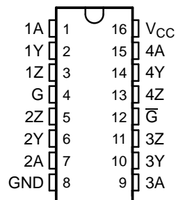
D OR NS PACKAGE (TOP VIEW)
