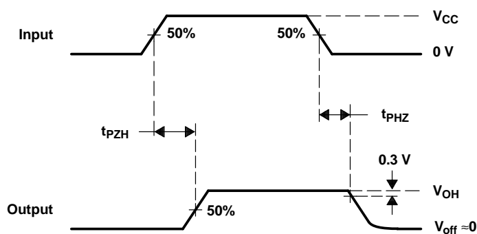
VOLTAGE WAVEFORMS
