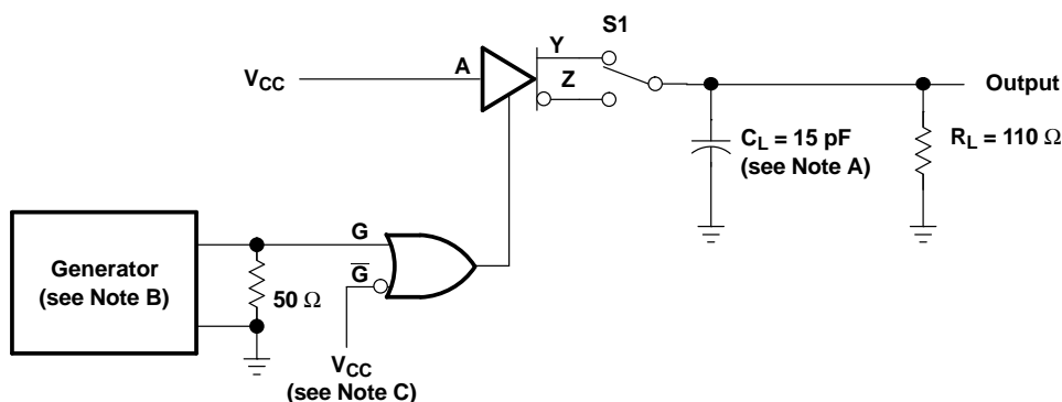
TEST CIRCUIT
