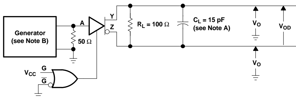
TEST CIRCUIT
