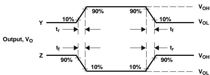
RISE AND FALL TIMES
