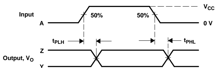
PROPAGATION DELAY TIMES
