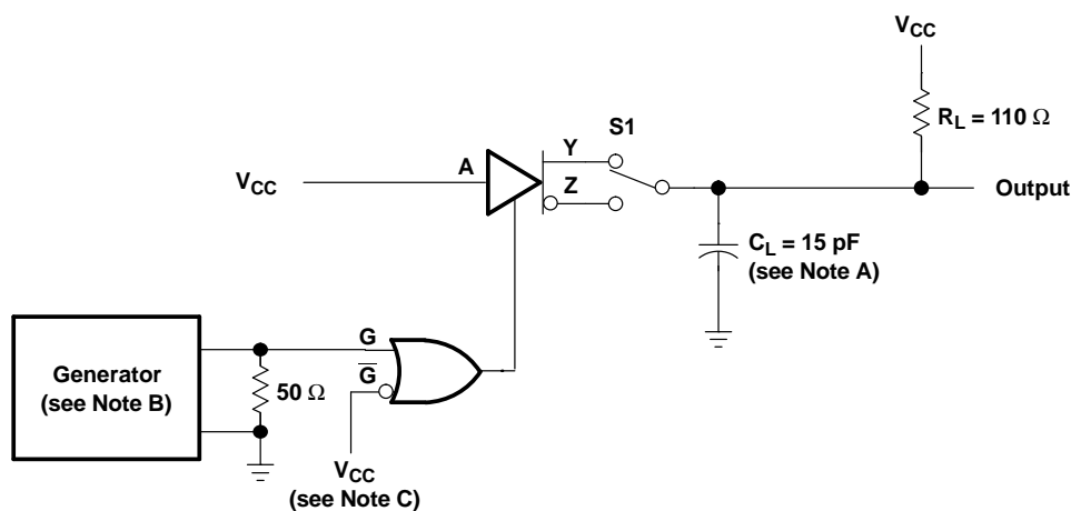
TEST CIRCUIT
