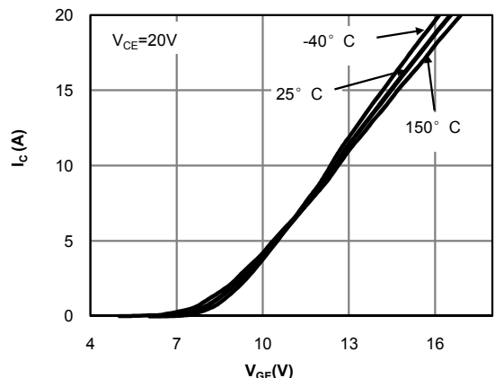
Fig 3: Transfer Characteristic
