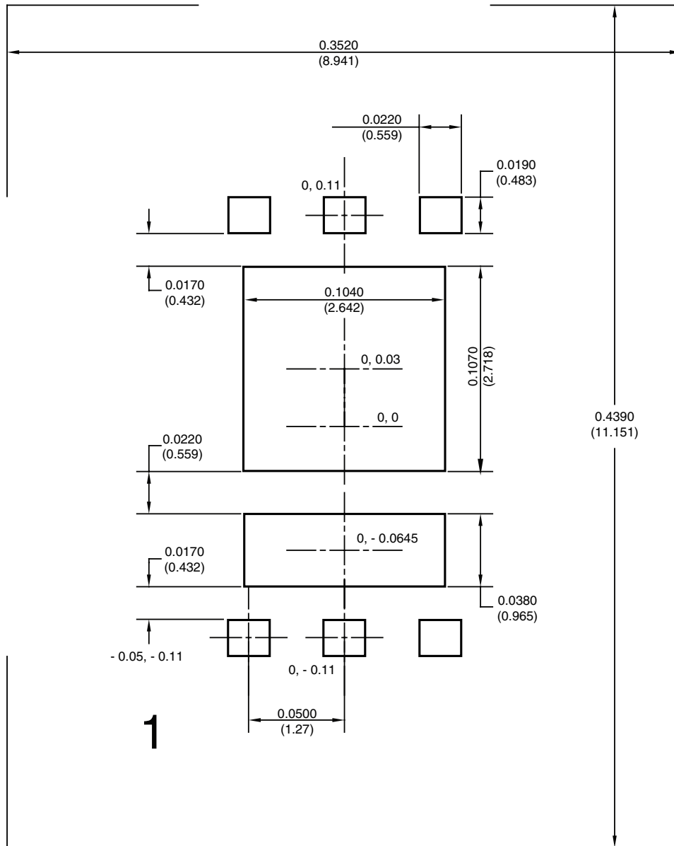
Recommended PAD for PowerPAIR 6 x 3.7 Dimensions in inches (mm) Keep-out 0.3520 (8.94) x 0.4390 (11.151)
