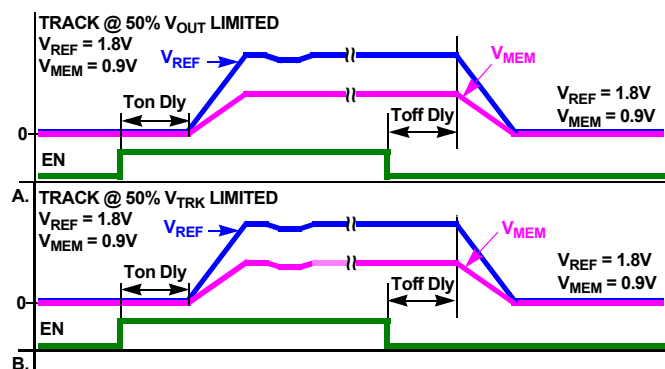
FIGURE 19. RATIOMETRIC TRACKING
