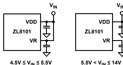
FIGURE 8. INPUT SUPPLY CONNECTIONS
