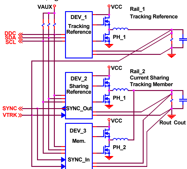
FIGURE 20. TRACKING CURRENT SHARING RAIL
