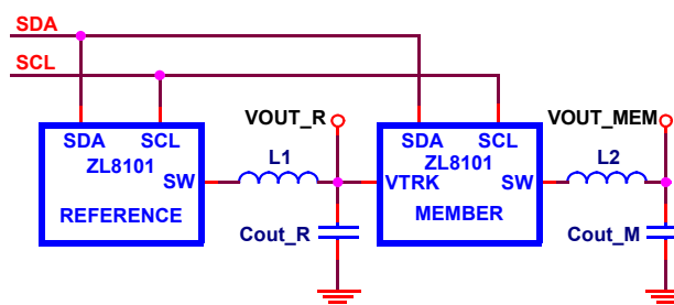
FIGURE 17. PMBus TRACKING
