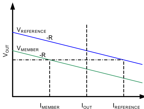
FIGURE 22. ACTIVE CURRENT SHARING
