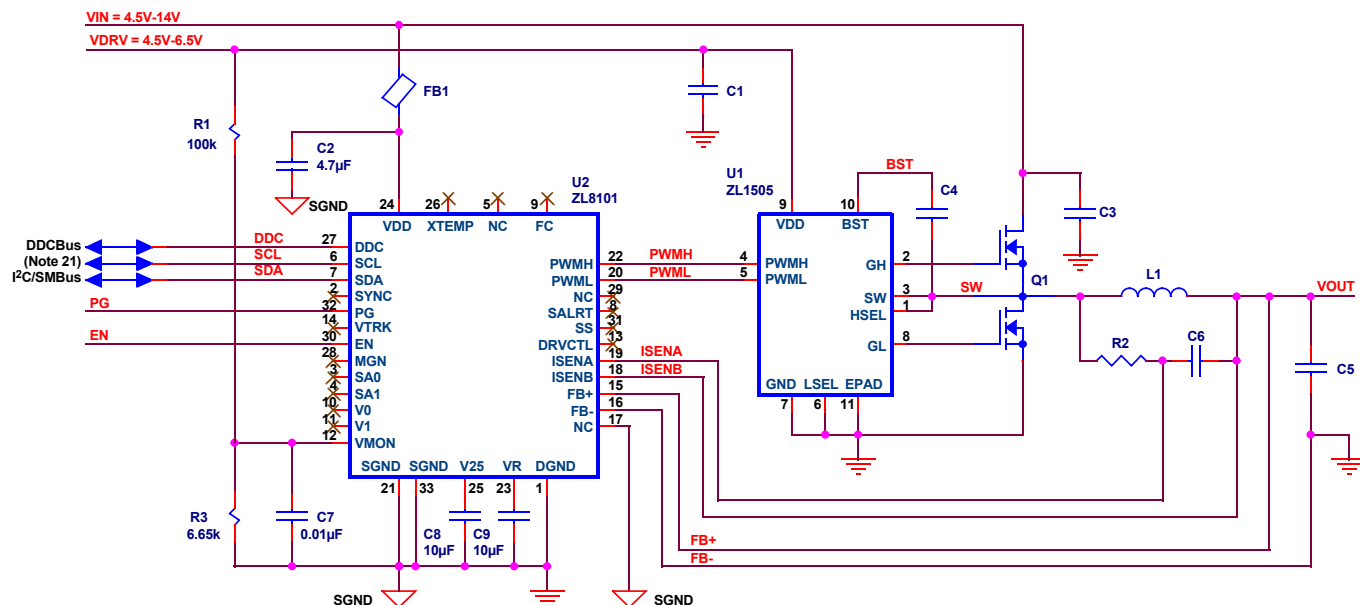
FIGURE 2. EXAMPLE DESIGN USING ZL8101 AND ZL1505 DRIVER
