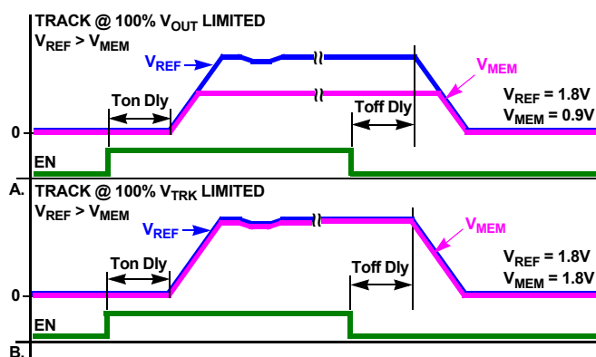
FIGURE 18. COINCIDENT TRACKING
