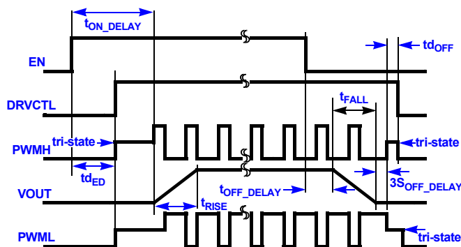
FIGURE 6. DRVCTL AND TRI-STATE BEHAVIOR
