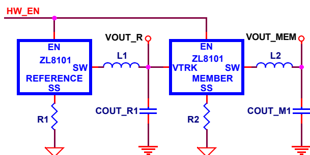
FIGURE 16. PINSTRAP TRACKING
