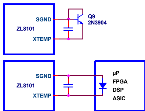
Embedded Thermal Diode FIGURE 25. XTEMP PIN CONNECTION
