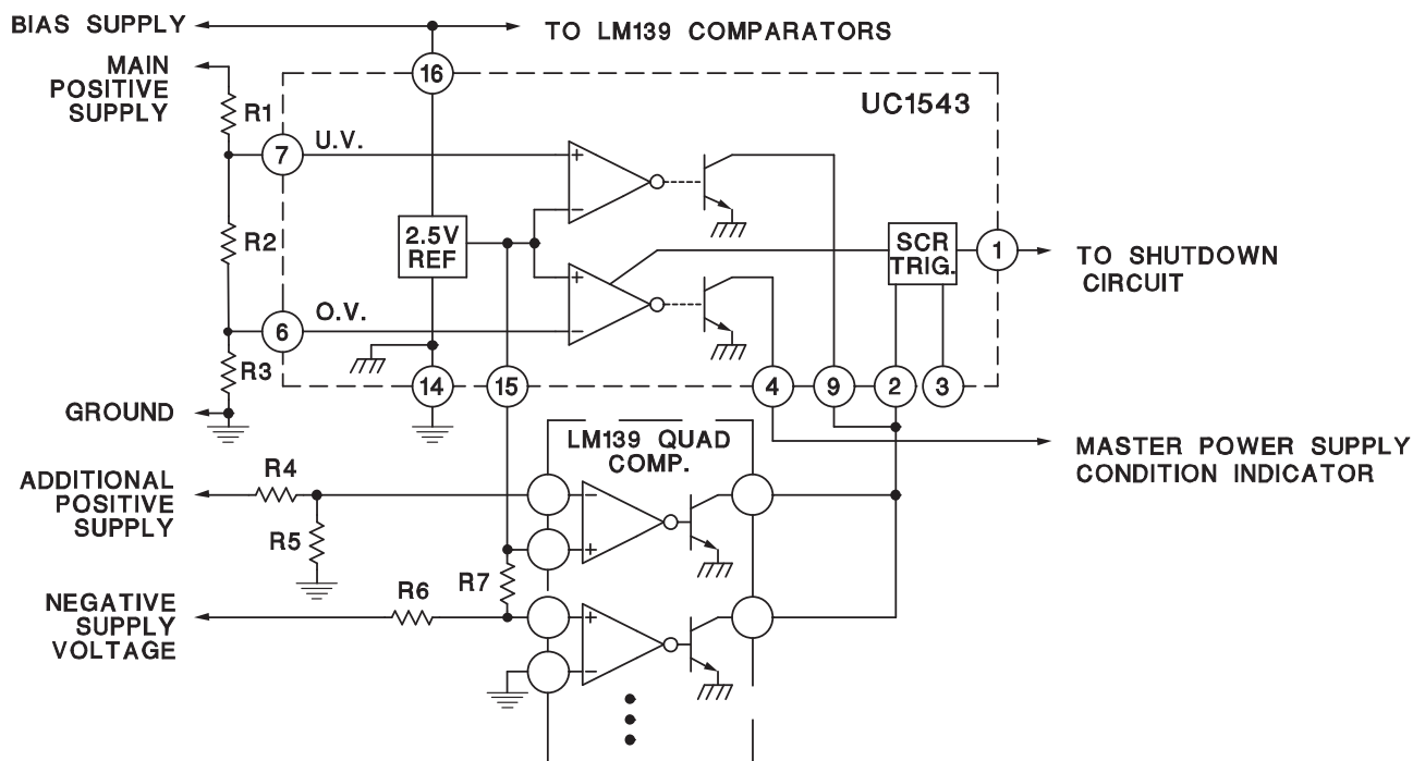
Figure 8. Sensing Multiple Supply Voltages
