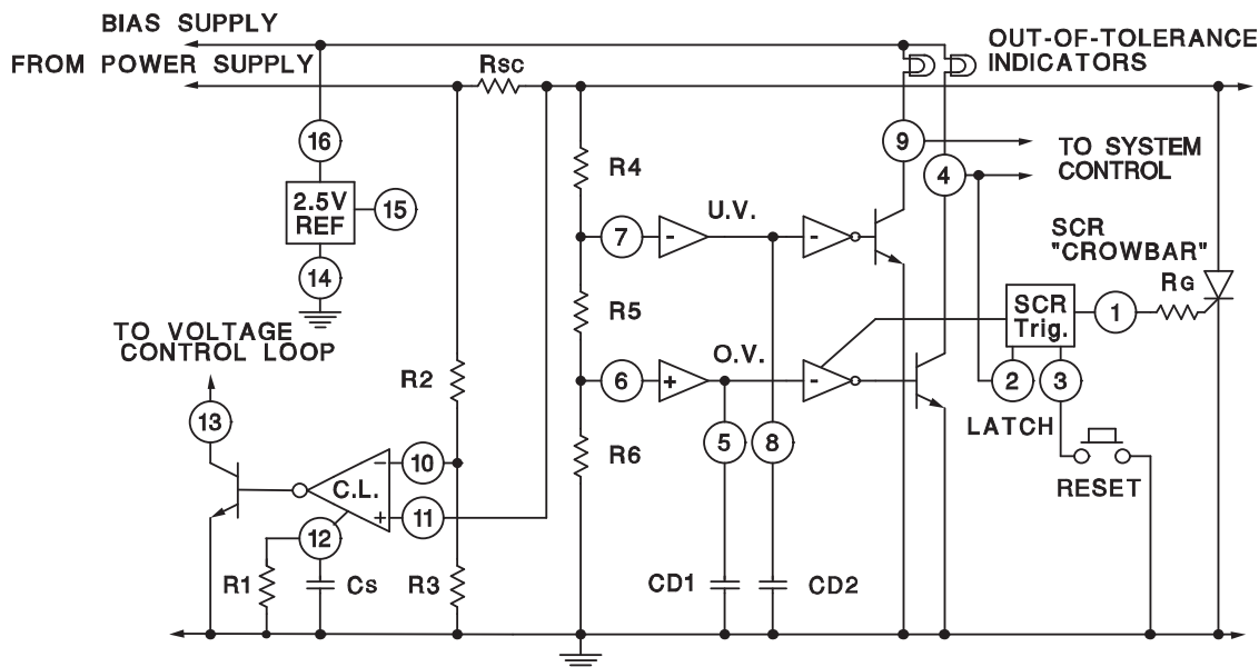
Figure 7. Typical Application
