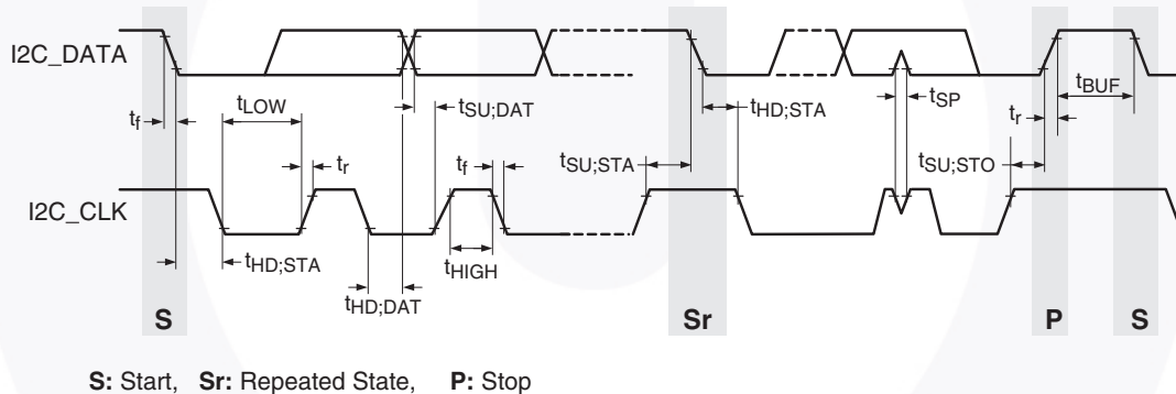
Figure 3. I 2 C Timing Diagram
