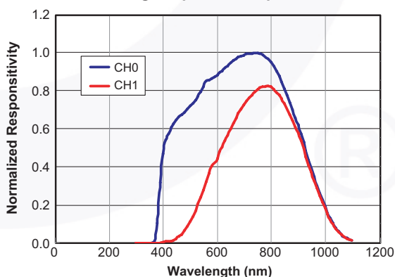
Fig. 2 Spectral Response
