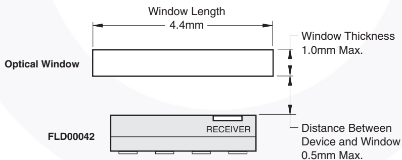
Side View of Recommended Mounting
