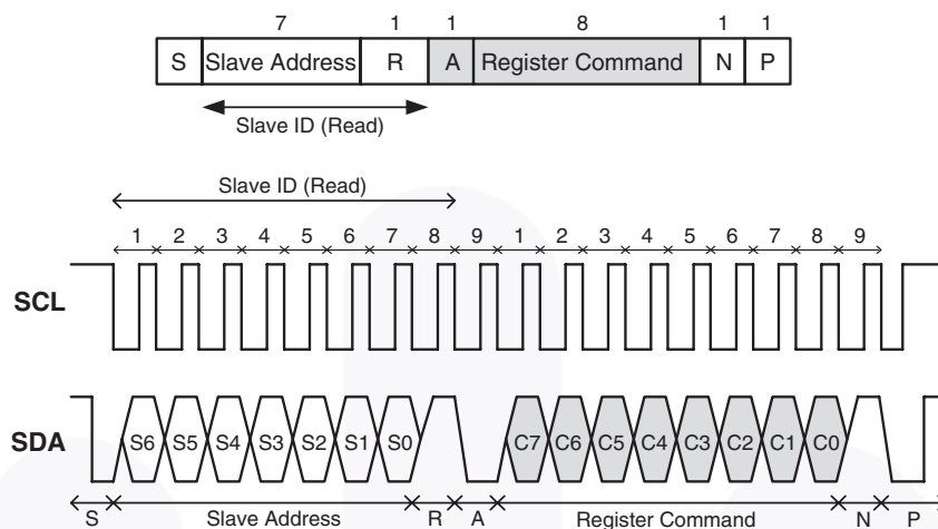
Figure 6. I 2 C Read Protocol
