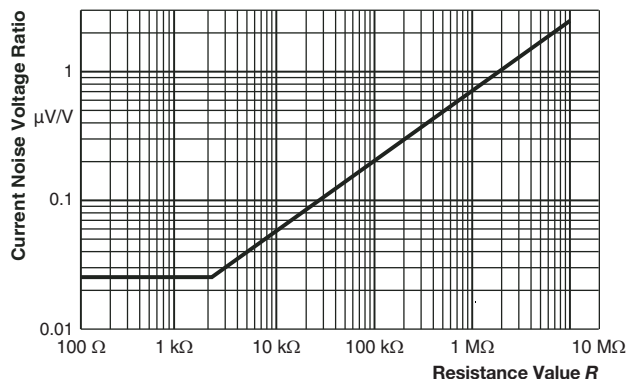
Current Noise Voltage Ratio
