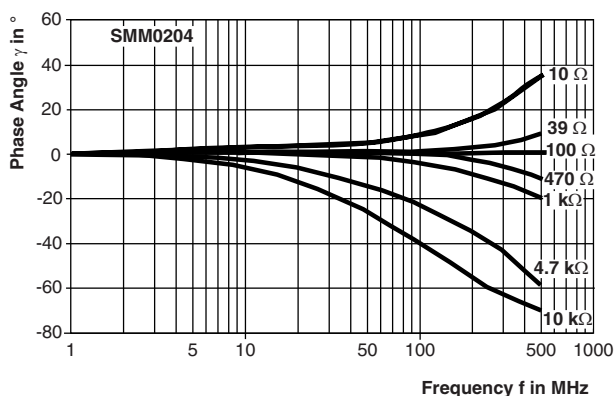
HF - Performance
