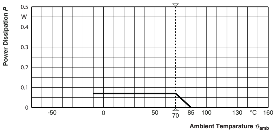
Derating - Precision Operation
