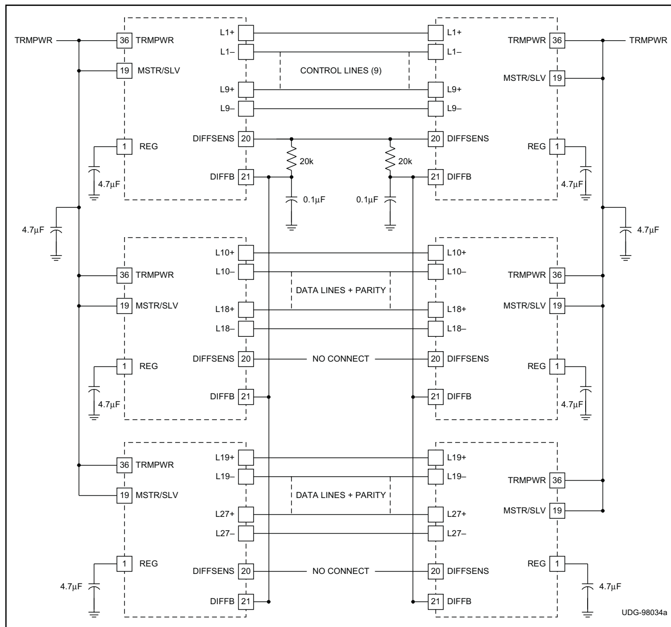
Figure 1. Application Drawing
