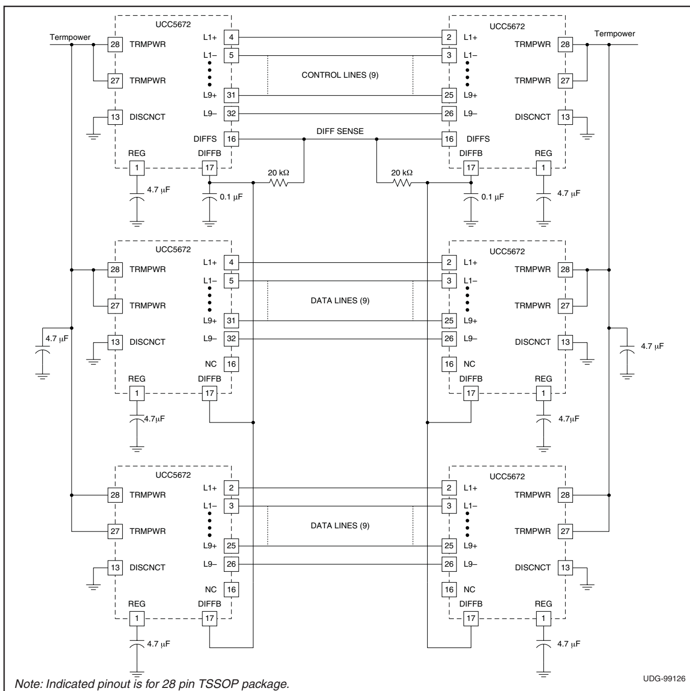
Figure 1. Application diagram.
