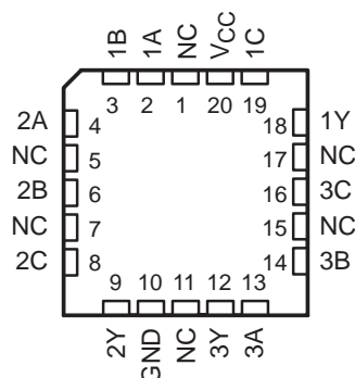
SN54F27 . . . FK PACKAGE (TOP VIEW)
