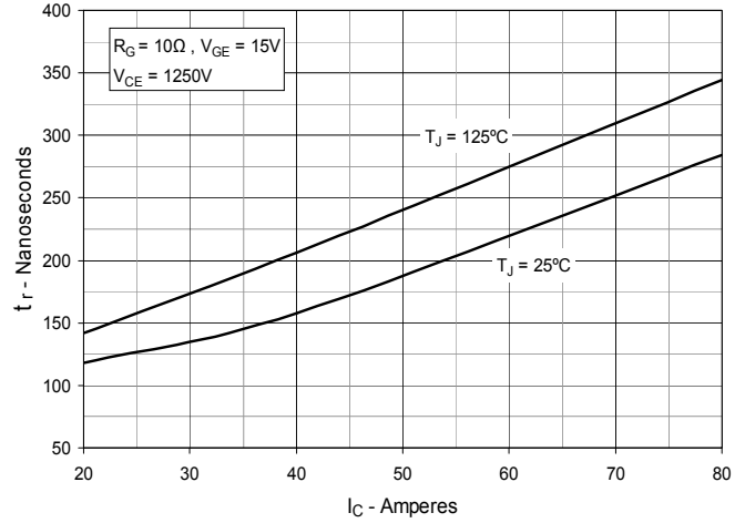
Fig. 13. Resistive Turn-on Rise Time vs. Collector Current
