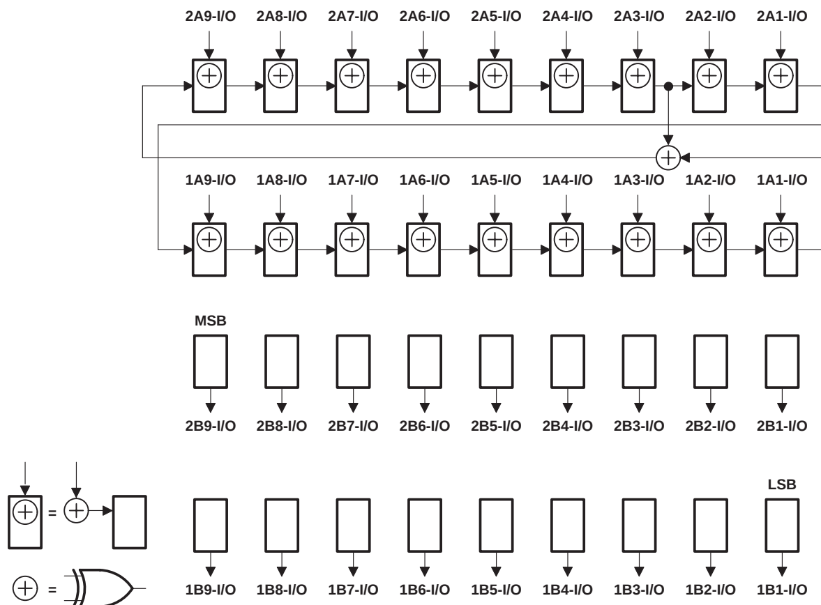
Figure 11. 18-Bit PSA/COUNT Configuration ( \overline{1OEAB} = \overline{2OEAB} = 0 , \overline{1OEB\overline{A}} = \overline{2OEB\overline{A}} = 1 )
