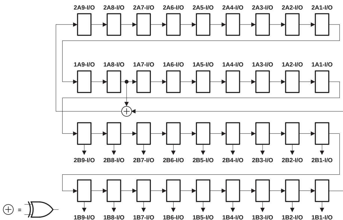
Figure 5. 36-Bit PRPG Configuration ( \overline{1OEAB} = \overline{2OEAB} = 0 , \overline{1OEBA} = \overline{2OEBA} = 1 )
