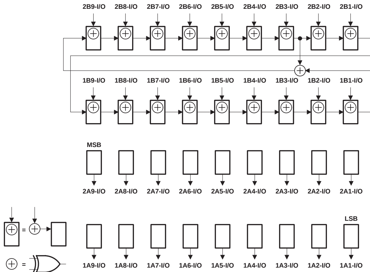
Figure 12. 18-Bit PSA/COUNT Configuration ( \overline{1OEAB} = \overline{2OEAB} = 1 , \overline{1OEBA} = \overline{2OEBA} = 0 )
