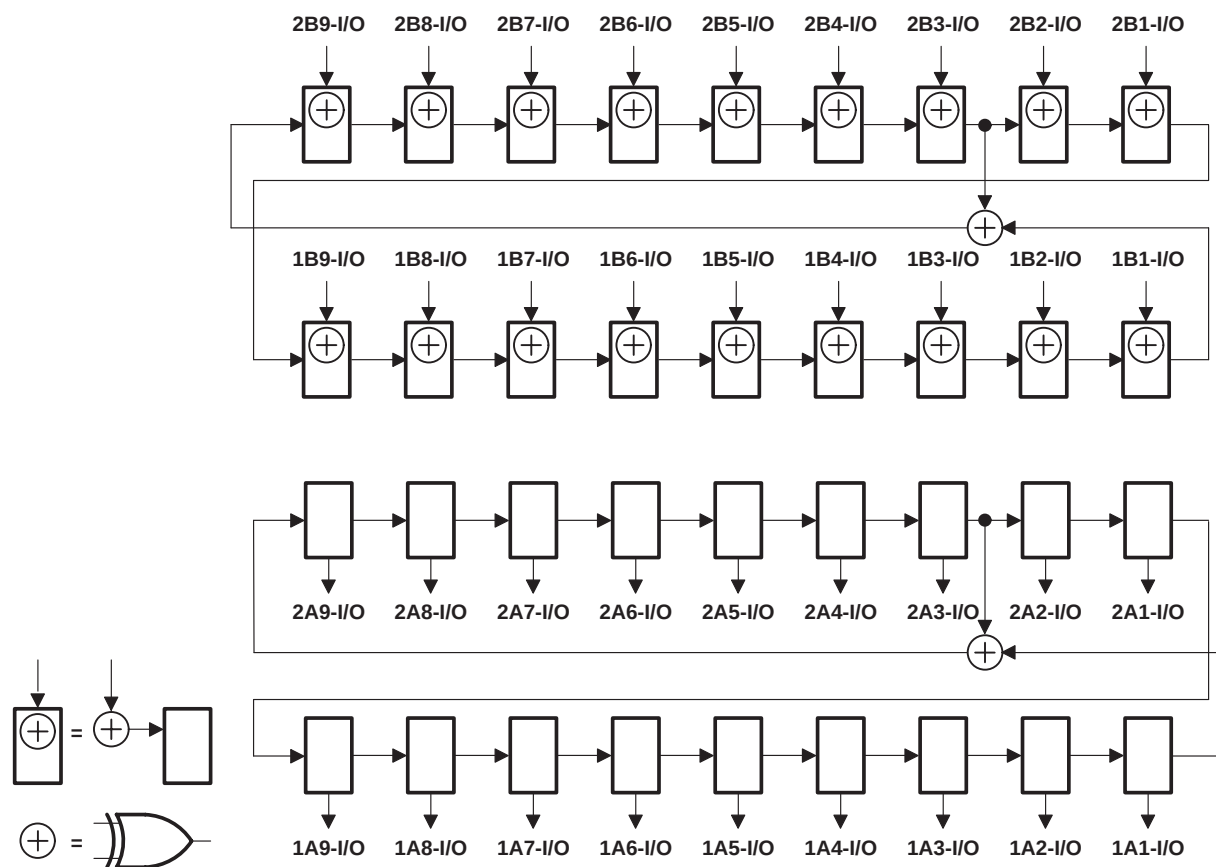
Figure 10. 18-Bit PSA/PRPG Configuration ( \overline{1OEAB} = \overline{2OEAB} = 1 , \overline{1OEBA} = \overline{2OEBA} = 0 )
