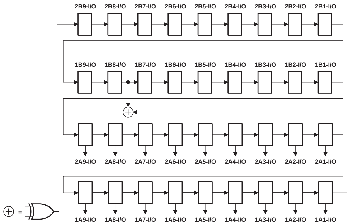
Figure 6. 36-Bit PRPG Configuration ( \overline{1OEAB} = \overline{2OEAB} = 1 , \overline{1OEBA} = \overline{2OEBA} = 0 )
