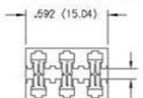
THREE OR SIX CONTACT ASSEMBLY
