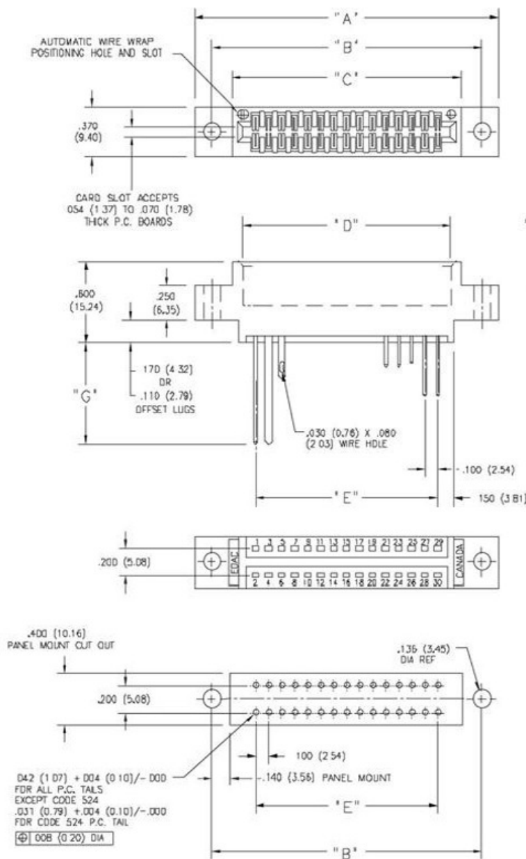
CONNECTOR MOUNTING PATTERN
