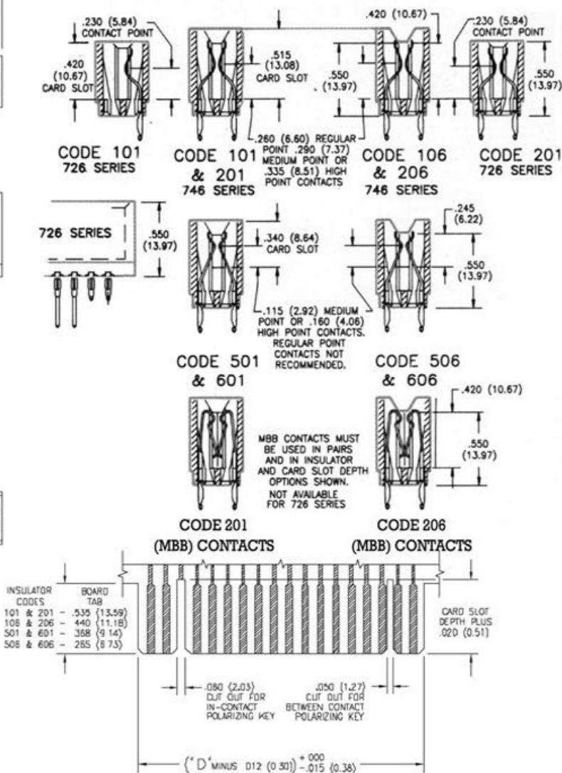
RECOMMENDED DAUGHTER BOARD
