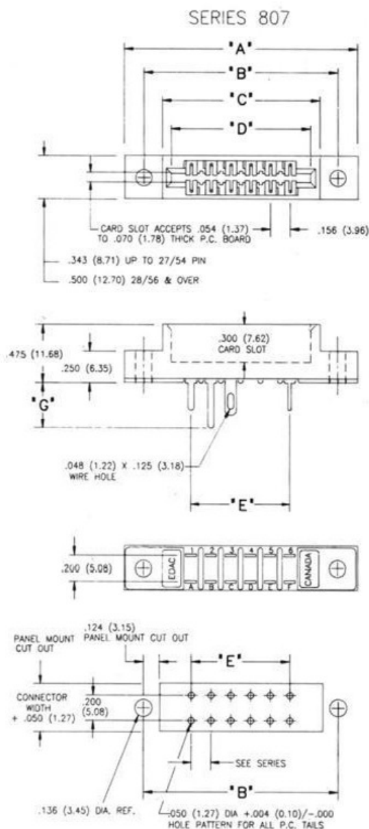
CONNECTOR MOUNTING PATTERN ALL SERIES
