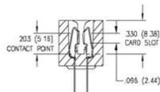
SECTION THROUGH CONTACT POSITION
