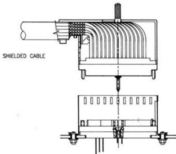
STANDARD EDAC 516 SERIES PLUG OR RECEPTACLE CONNECTOR WITH SHIELDING HARDWARE IN PLACE
