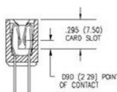
INSULATOR STYLE CODE 2
