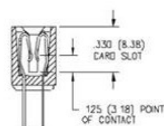
INSULATOR STYLE CODE 5
