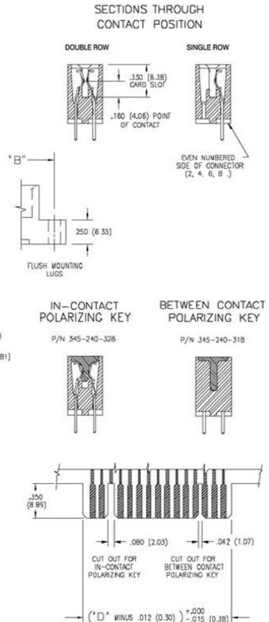
RECOMMENDED DAUGHTER BOARD
