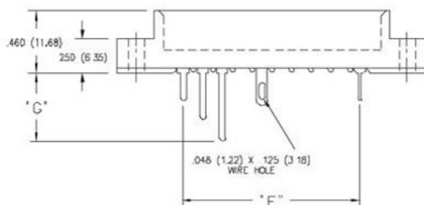
INSULATOR STYLE CODE 2
