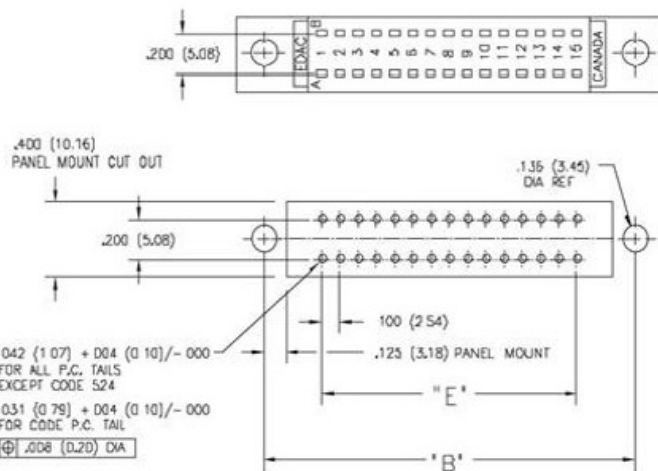
CONNECTOR MOUNTING PATTERN
