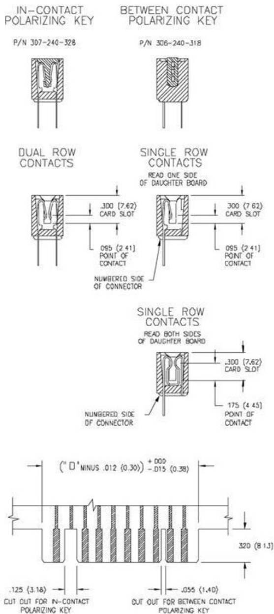
RECOMMENDED DAUGHTER BOARD
