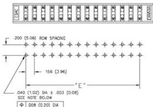
RECOMMENDED MOTHER BOARD HOLE PATTERN
