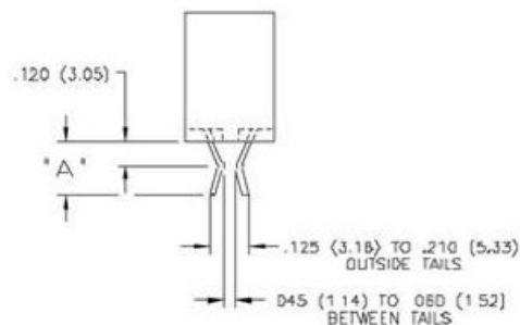
CONTACT CODE 555 BEND USES WIRE HOLE CONTACTS
