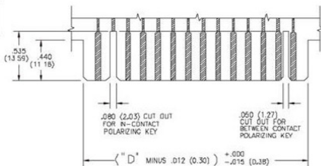
RECOMMENDED DAUGHTER BOARD
