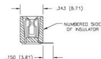
CONTACT CODE 554 BEND USES WIRE HOLE CONTACTS
