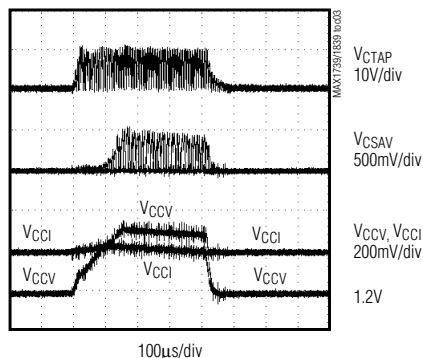
WIDE INPUT RANGE ( V_{BATT} = 8V , DPWM = 9\% , V_{CTL} = 0 )
