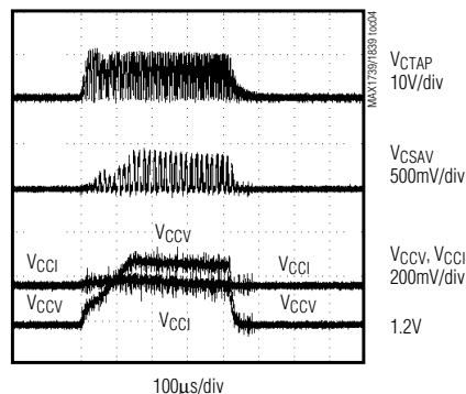
WIDE INPUT RANGE ( V_{BATT} = 20V , DPWM = 9\% , V_{CTL} = 0 )
