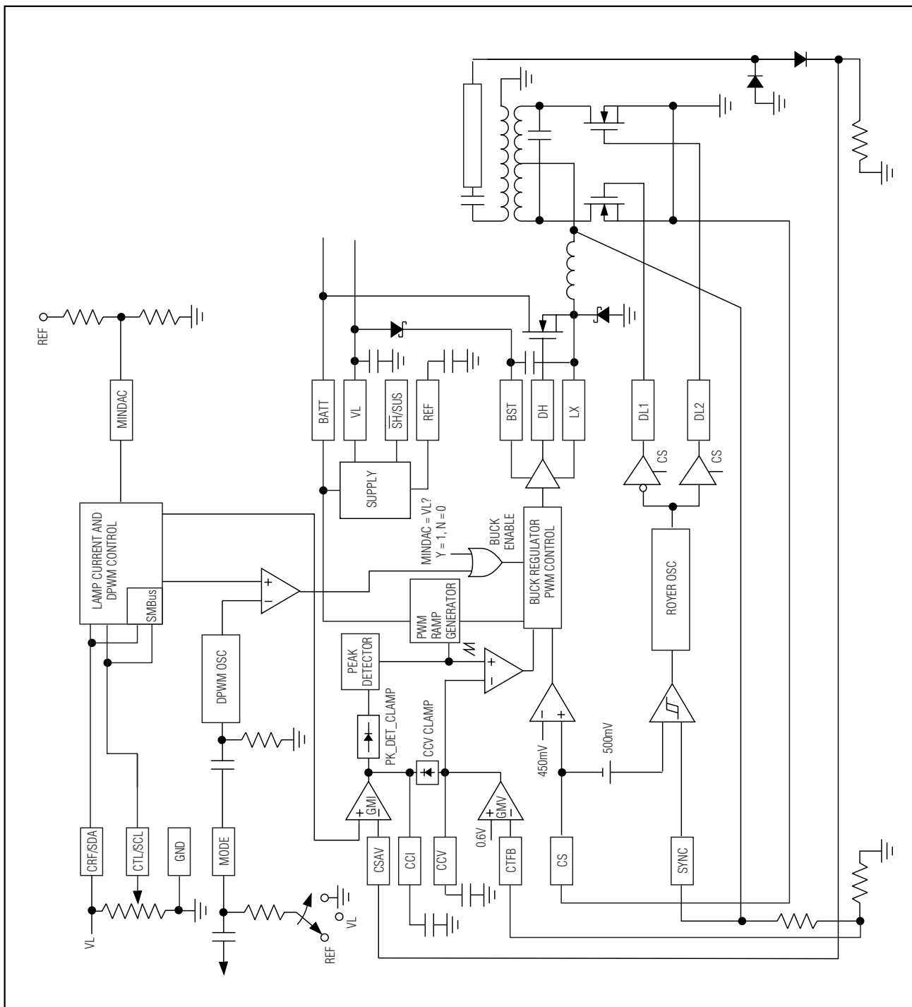
Figure 2. Functional Diagram
