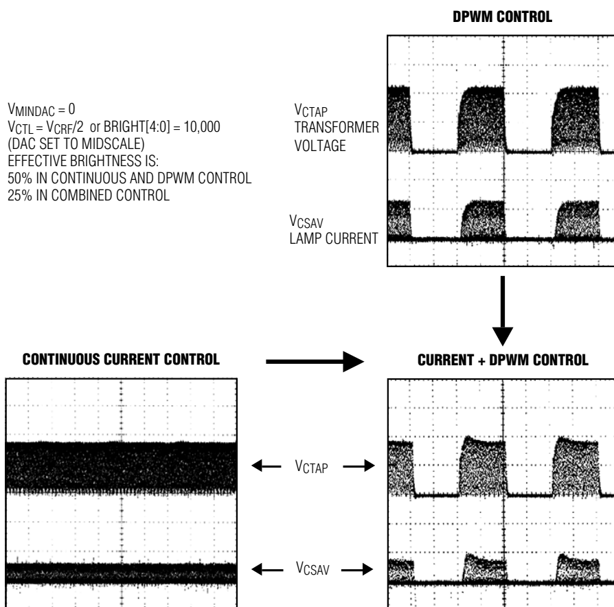
Figure 1. Brightness Control Methods
