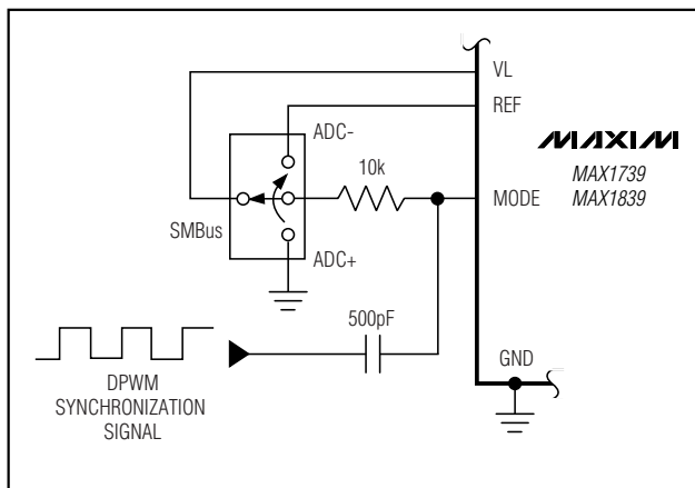
Figure 6. DPWM Synchronization
