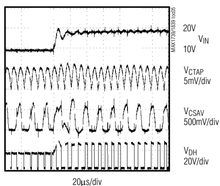
FEED-FORWARD COMPENSATION
