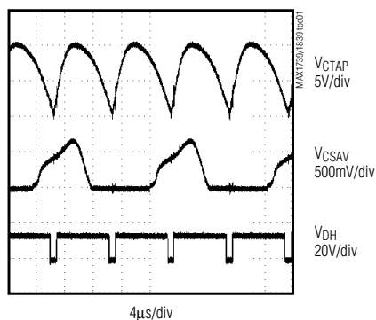
WIDE INPUT RANGE ( V_{BATT} = 8V )
