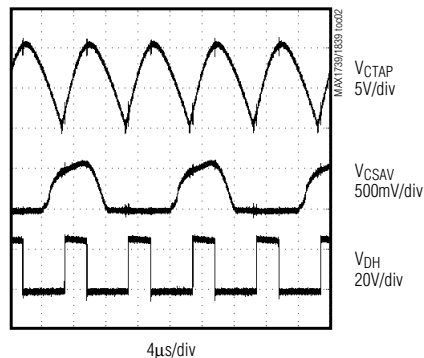
WIDE INPUT RANGE ( V_{BATT} = 20V )
