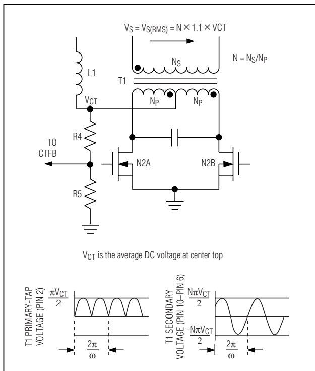
Figure 9. Transformer Primary/Secondary Voltage Relationship
