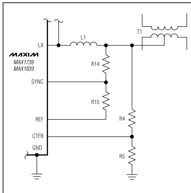
Figure 7. Adjusting the ZVC Detection
