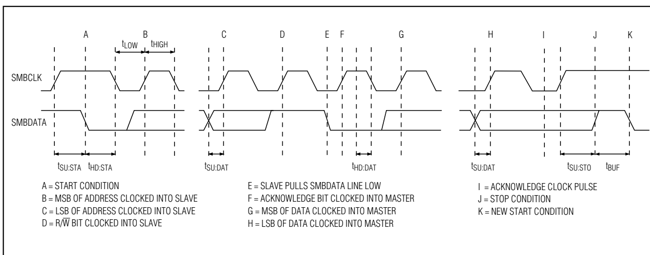
Figure 13. SMBus Read Timing
