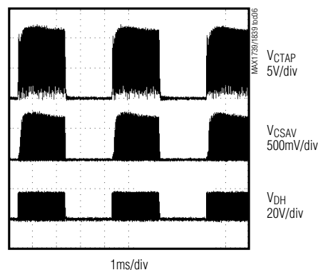
SYNCHRONIZED DPWM ( f_{MODE} = 32kHz , V_{CTL} = V_{CRF}/2 )
