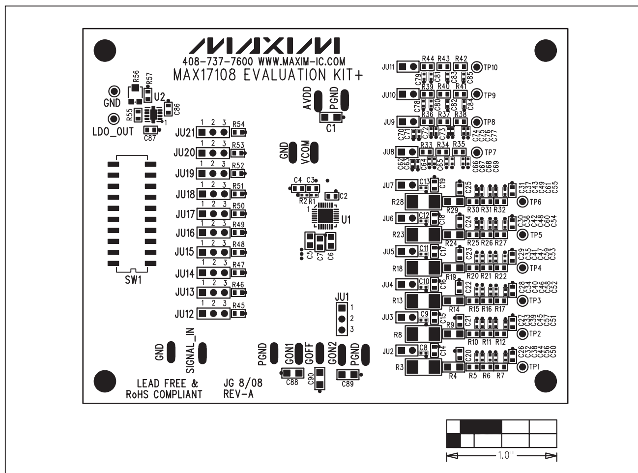
Figure 2. MAX17108 EV Kit Component Placement Guide—Component Side
