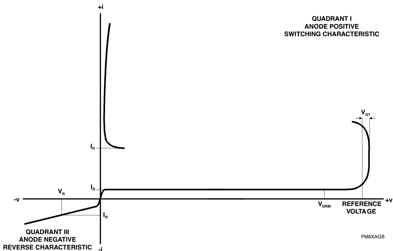
Figure 1. Voltage-Current Characteristic
