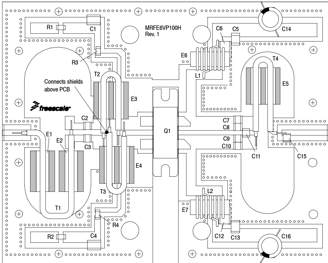
Figure 11. MRFE6VP100HR5(HSR5) Broadband Reference Circuit Component Layout — 30-512 MHz
