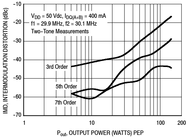
Figure 18. Intermodulation Distortion Products versus Output Power — 30 MHz
