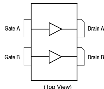
Figure 1. Pin Connections
