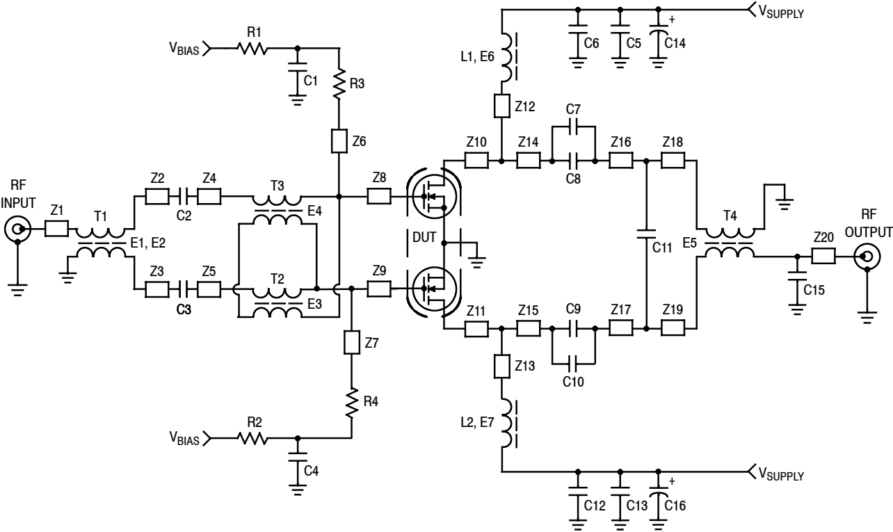
Figure 12. MRFE6VP100HR5(HSR5) Broadband Test Circuit Schematic — 30-512 MHz
