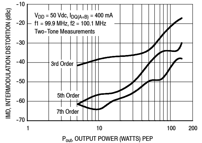
Figure 19. Intermodulation Distortion Products versus Output Power — 100 MHz
