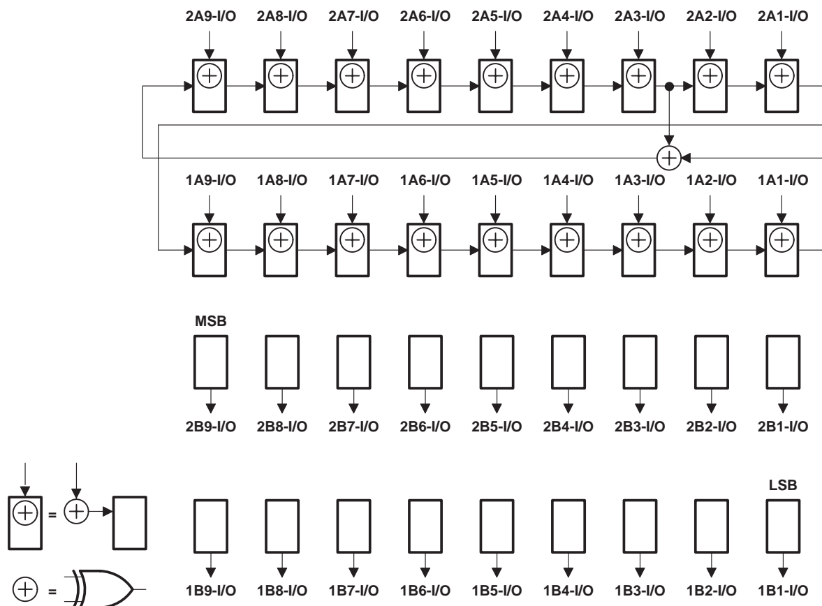
Figure 11. 18-Bit PSA/COUNT Configuration ( \overline{1OEAB} = \overline{2OEAB} = 0 , \overline{1OEB\bar{A}} = \overline{2OEB\bar{A}} = 1 )
