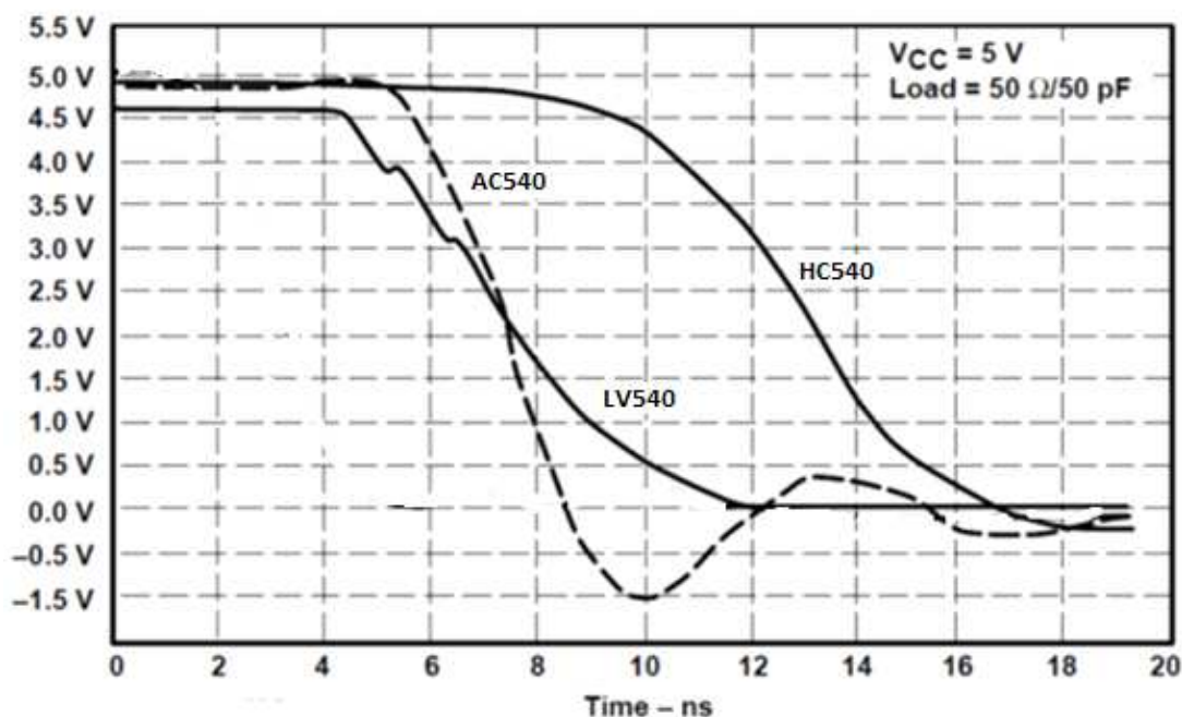
Figure 5. Switching Characteristics Comparison
