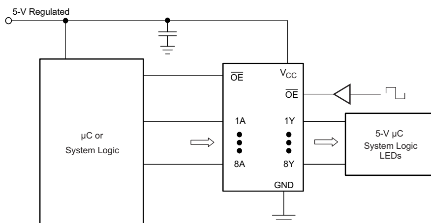
Figure 4. Typical Application Schematic
