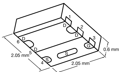
Thin PowerPAK SC-70-6L-Single
