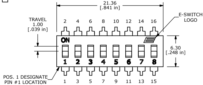
P.C.B. MOUNTING
