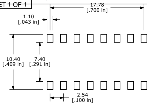
P.C.B. MOUNTING
