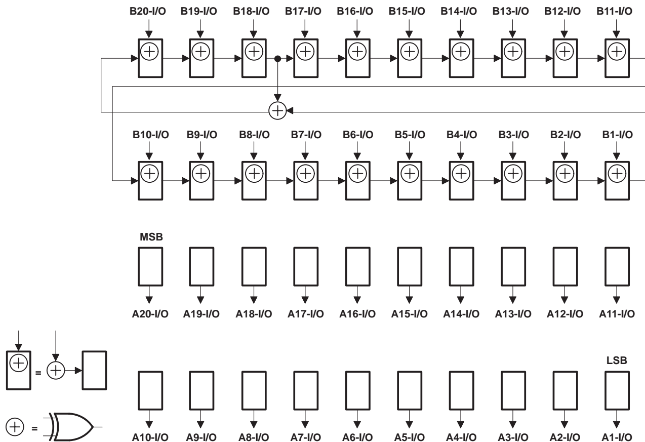
Figure 12. 20-Bit PSA/COUNT Configuration ( \overline{\text{OEAB}} = 1 , \overline{\text{OEBA}} = 0 )
