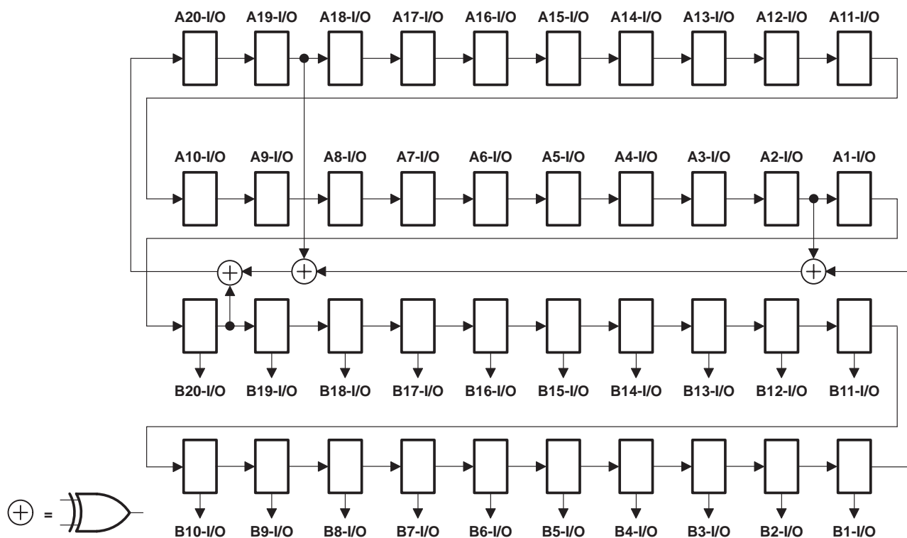
Figure 5. 40-Bit PRPG Configuration ( \overline{\text{OEAB}} = 0 , \overline{\text{OEBA}} = 1 )
