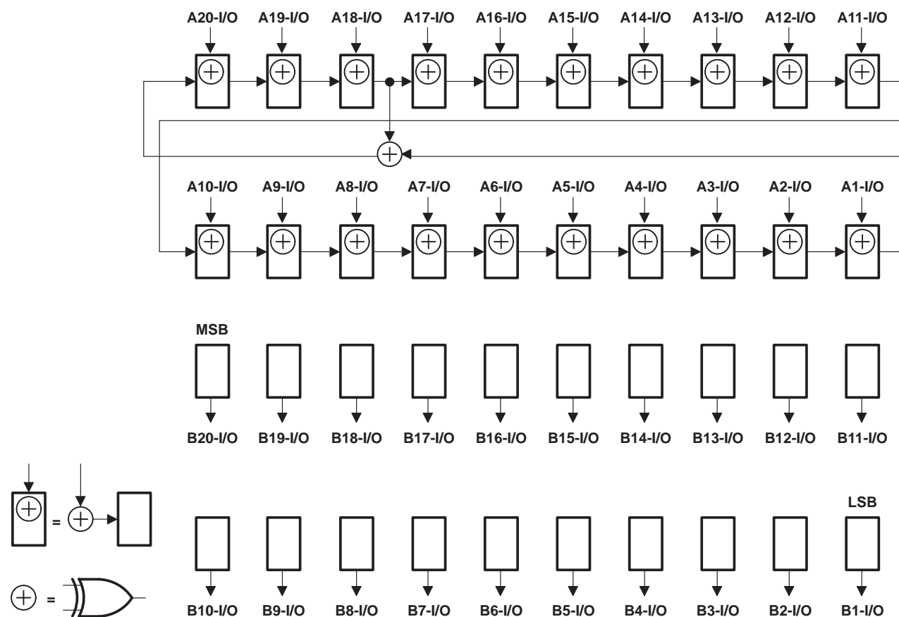
Figure 11. 20-Bit PSA/COUNT Configuration ( \overline{\text{OEAB}} = 0 , \overline{\text{OEBA}} = 1 )
