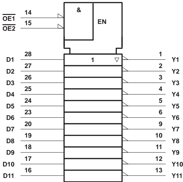
logic symbol†
