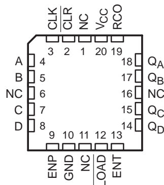
SN54HC161 . . . FK PACKAGE (TOP VIEW)
