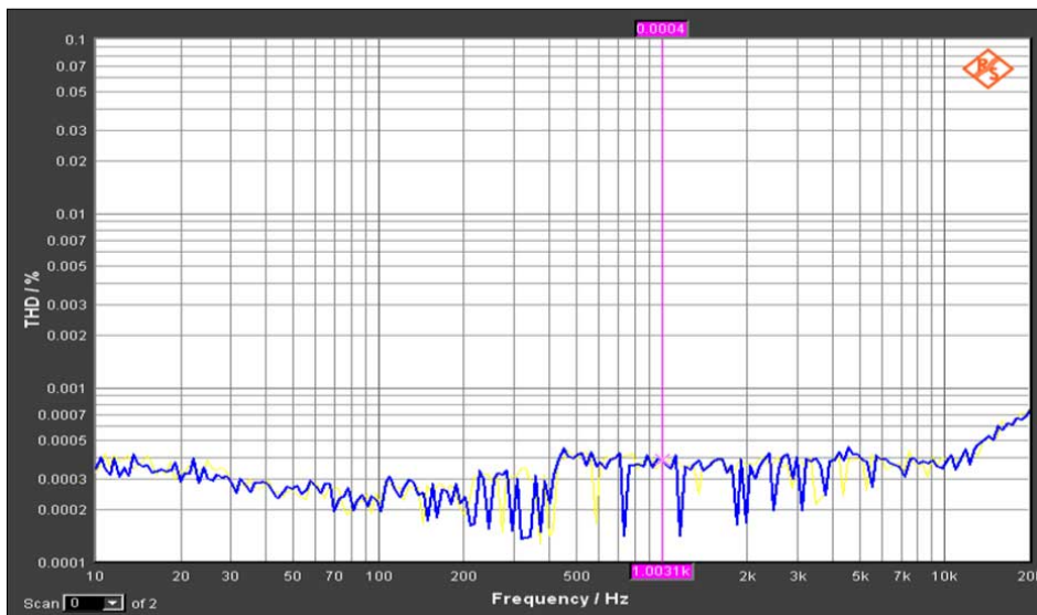
Figure 18. Total harmonic distortion on differential lanes
