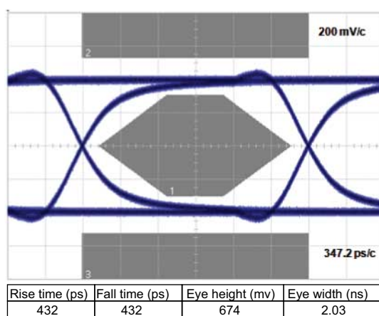
Figure 15. Eye diagram (loaded by Z diff = 90 Ω) with USB2.0 [mask 1] board with ECM02-4CMX8
