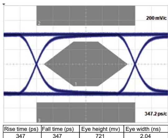
Figure 14. Eye diagram (loaded by Z diff = 90 Ω) with USB2.0 [mask 1] board only
