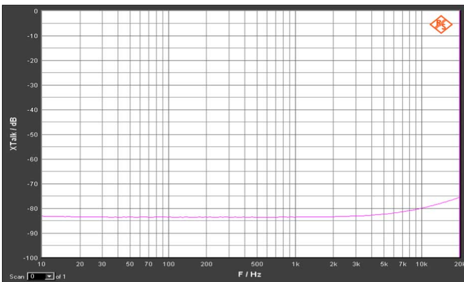
Figure 19. Crosstalk on differential lanes
