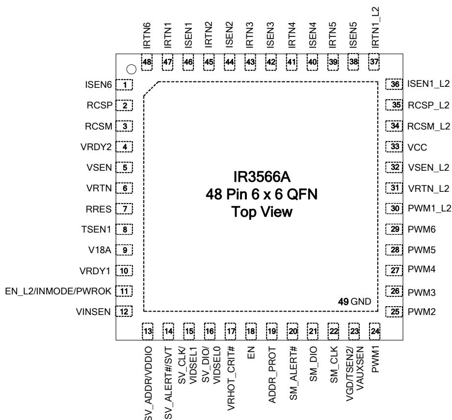
Figure 1: IR3566A Pin Diagram Enlarged
