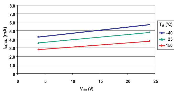
Supply Current (On) versus Supply Voltage (A1101/02/03/04/06)
