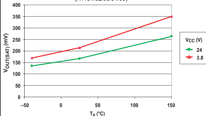
Output Voltage (On) versus Ambient Temperature (A1101/02/03/04/06)
