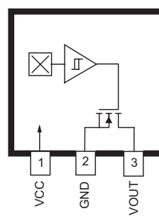
Package UA, 3-pin SIP
