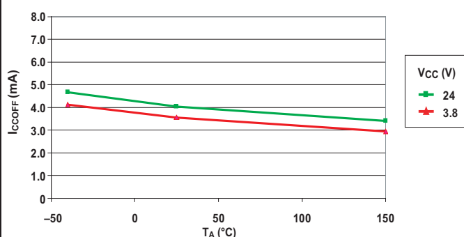
Supply Current (Off) versus Ambient Temperature (A1101/02/03/04/06)
