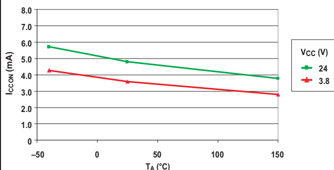
Supply Current (On) versus Ambient Temperature (A1101/02/03/04/06)
