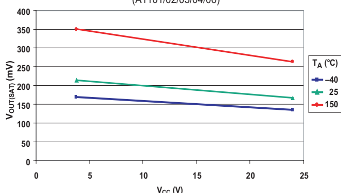
Output Voltage (On) versus Supply Voltage (A1101/02/03/04/06)
