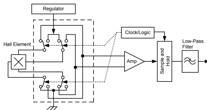
Chopper Stabilization Technique
