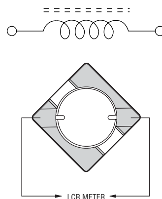
Electrical Schematic
