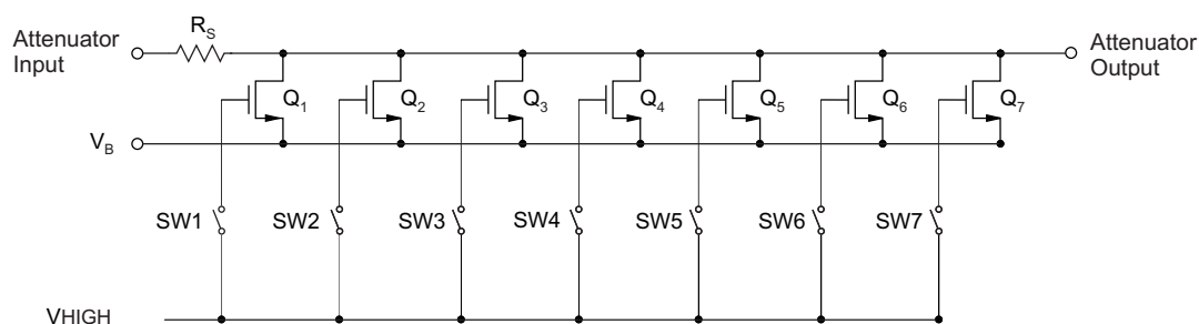
Figure 64. Simplified Voltage-Controlled Attenuator (Digital Structure)
