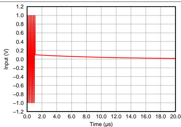
Figure 53. Pulse Inversion Asymmetrical Positive Input
