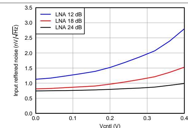
Figure 19. IRN, PGA = 24 dB and Low Noise Mode
