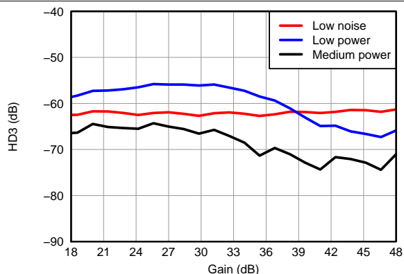
Figure 44. HD3 vs Gain, LNA = 24 dB and PGA = 24 dB and V_{\text{OUT}} = -1 dBFS
