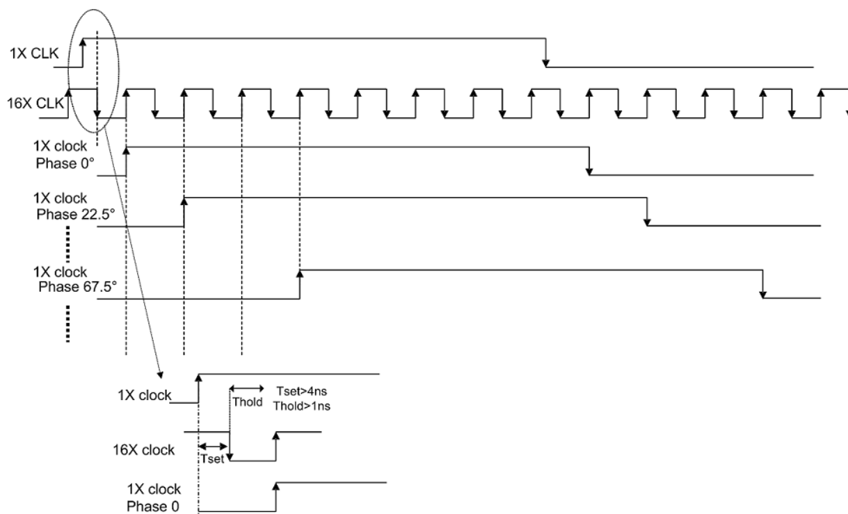
Figure 70. 1× and 16× CW Clock Timing
