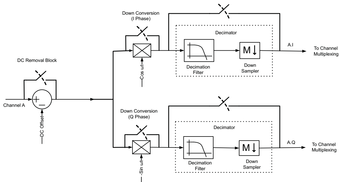
Figure 75. Digital Demodulator Block
