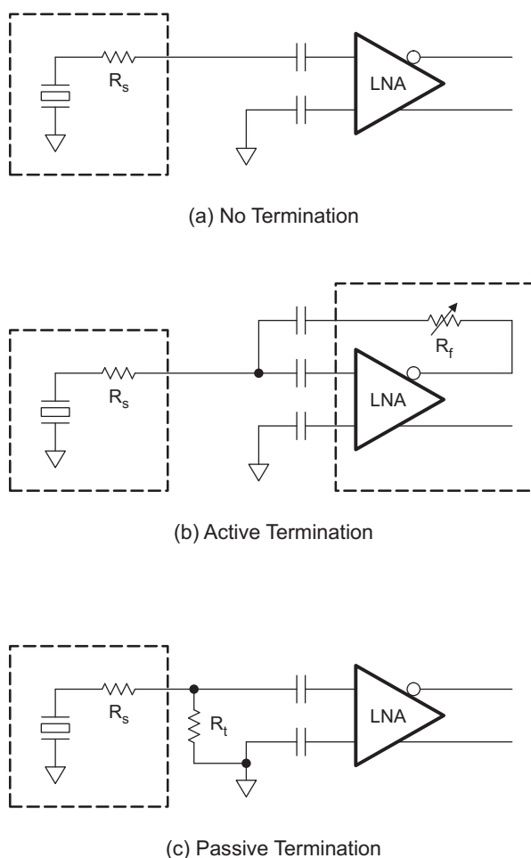
Figure 100. Termination Configurations
