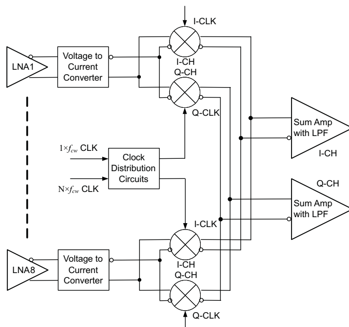
Figure 66. Simplified Block Diagram of CW Path
