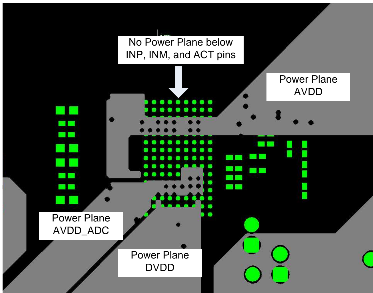
Figure 116. Layout Example
