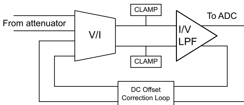
Figure 65. Simplified Block Diagram of PGA
