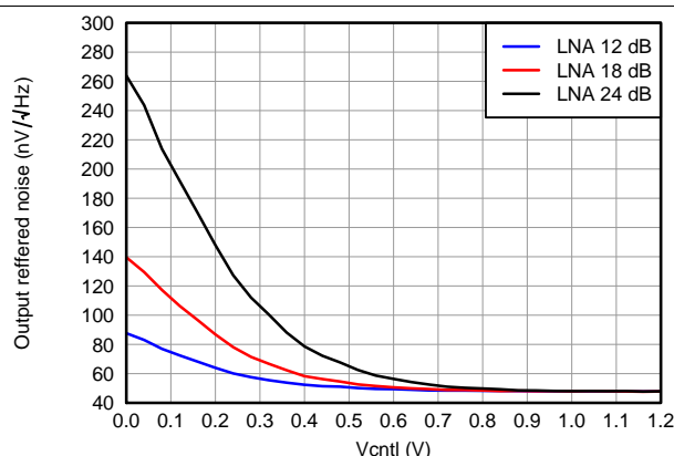
Figure 25. ORN, PGA = 24 dB and Medium-Power Mode
