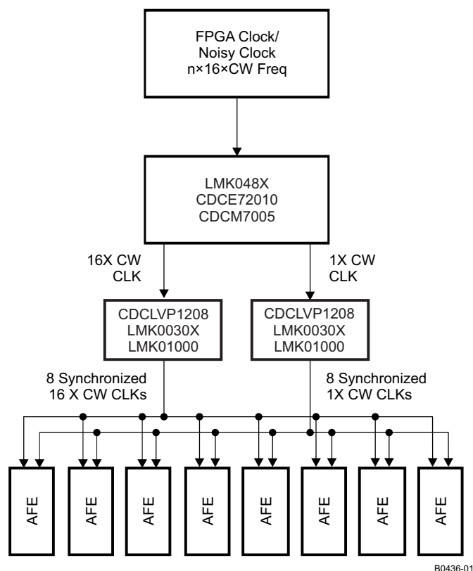
Figure 108. CW Clock Distribution
