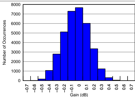
Figure 6. Gain Matching Histogram, V_{CNTL} = 0.9 V (34951 Channels)
