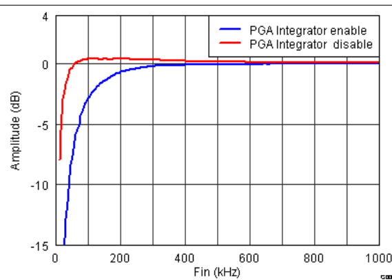
Figure 59. Signal Chain Low Frequency Response With INM Capacitor = 1 μF
