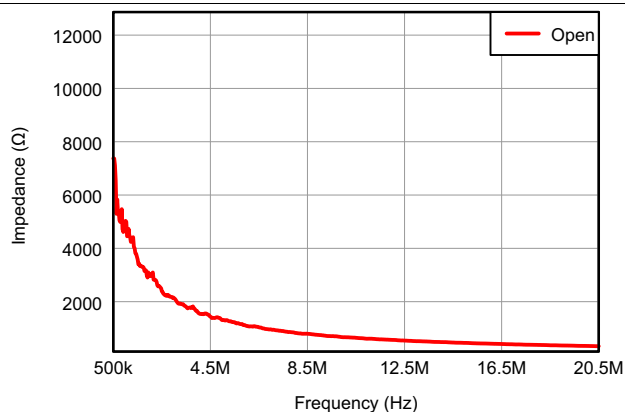
Figure 8. Input Impedance Without Active Termination (Magnitude)
