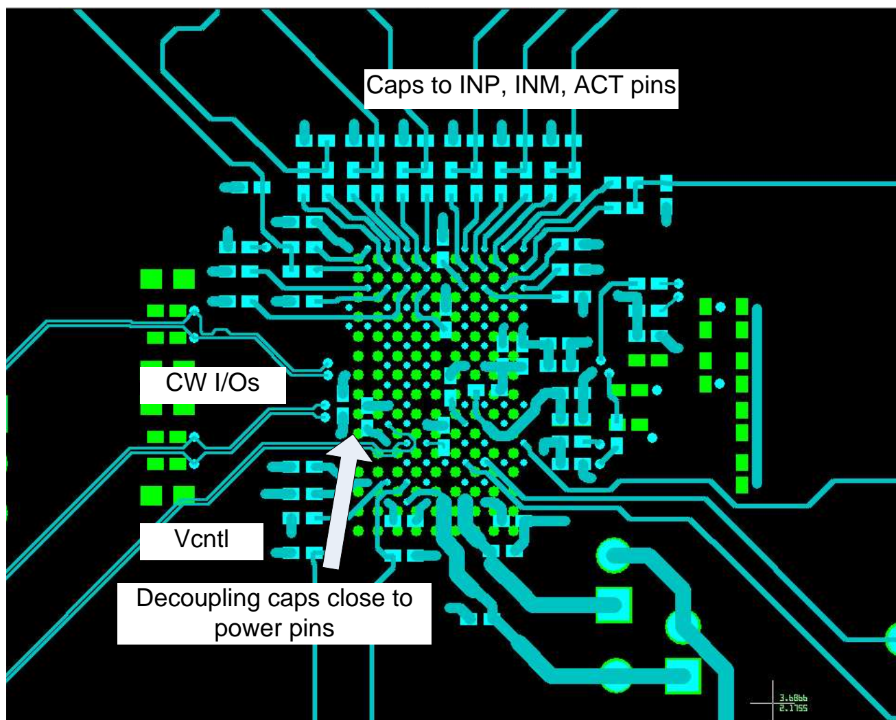
Figure 114. Layout Example
