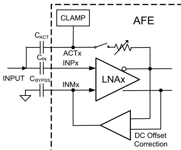
Figure 62. AFE5809 LNA With DC Offset Correction Circuit
