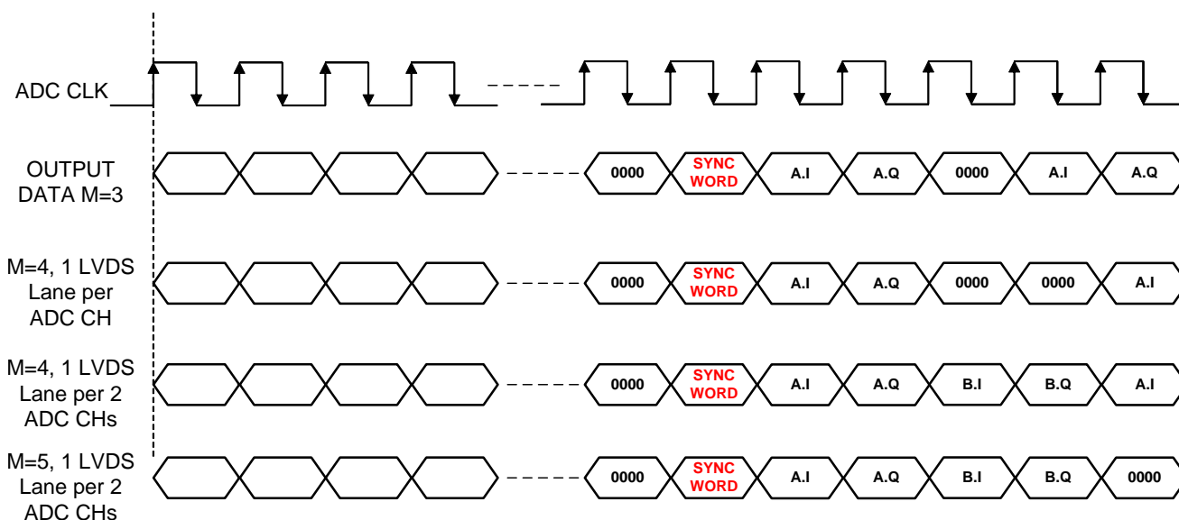
Figure 87. Output Data Format at M = 3~5
