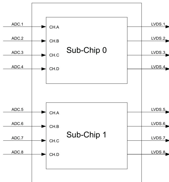
Figure 74. Subchip
