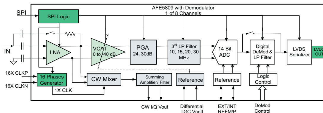
Figure 60. Simplified Functional Block Diagram
