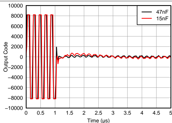
Figure 56. Overload Recovery Response vs INM Capacitor, V IN = 50 mVpp/100 μVpp, Max Gain
