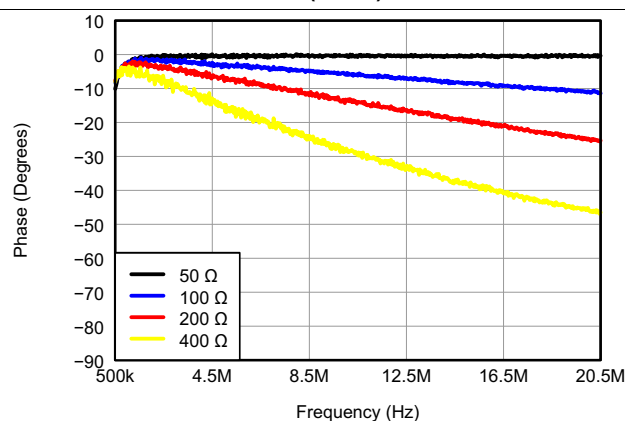
Figure 11. Input Impedance With Active Termination (Phase)
