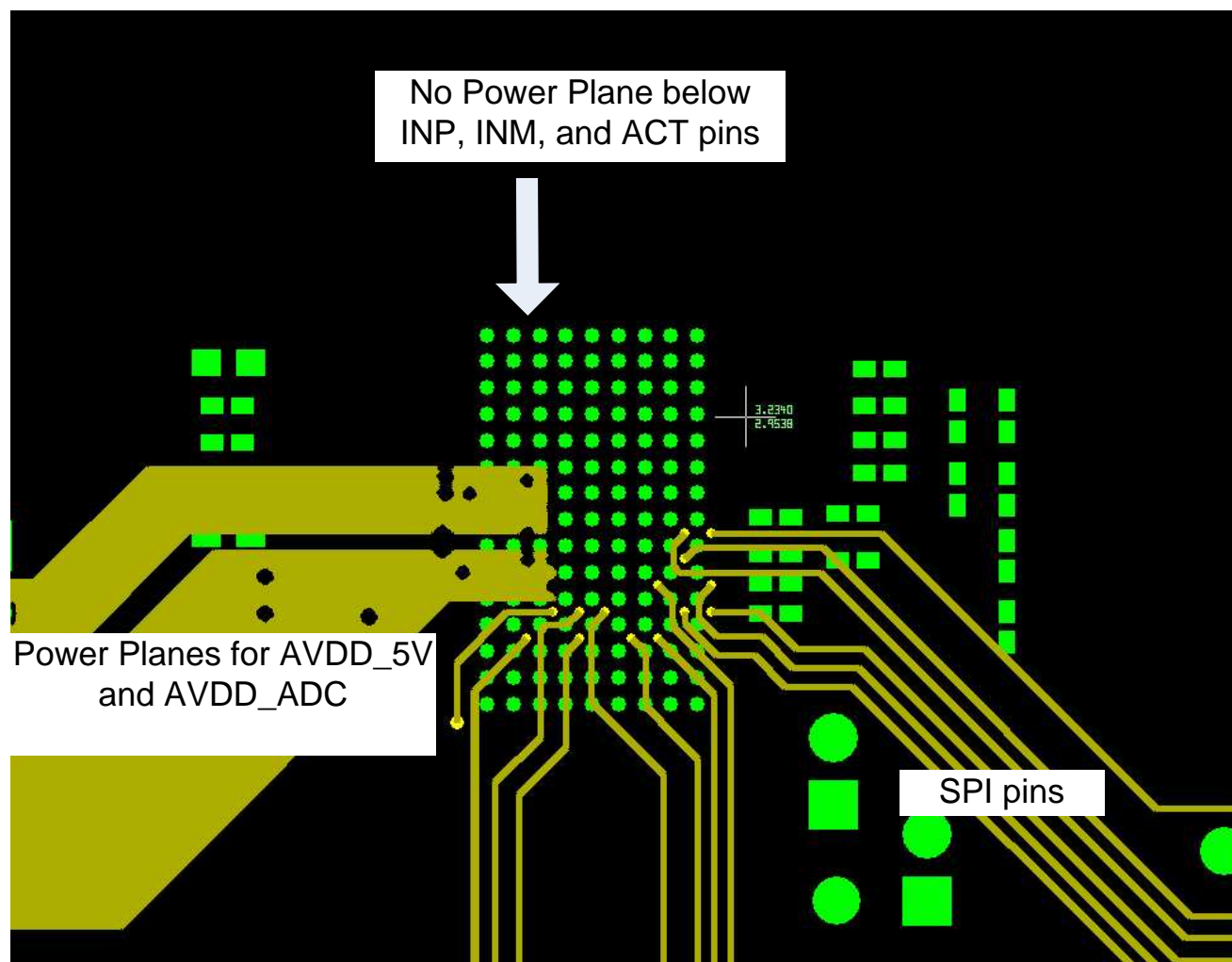
Figure 115. Layout Example
