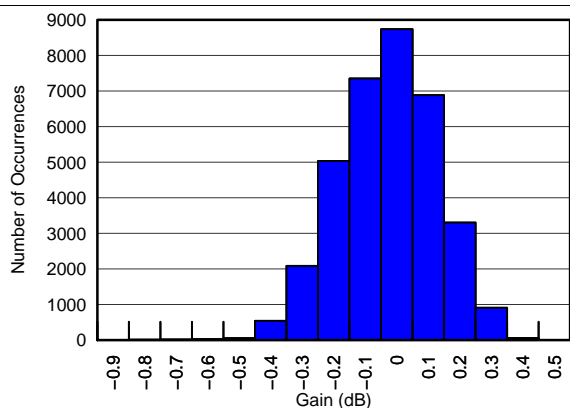
Figure 4. Gain Matching Histogram, V_{CNTL} = 0.3 V (34951 Channels)
