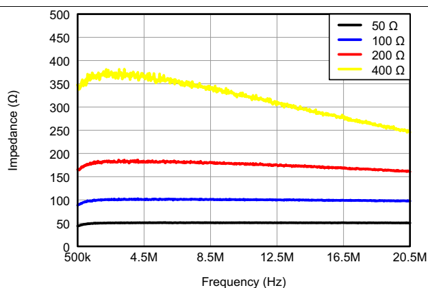
Figure 10. Input Impedance With Active Termination (Magnitude)
