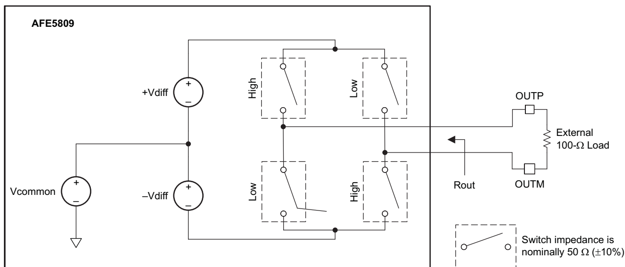
Figure 81. Equivalent Circuits of LVDS Outputs
