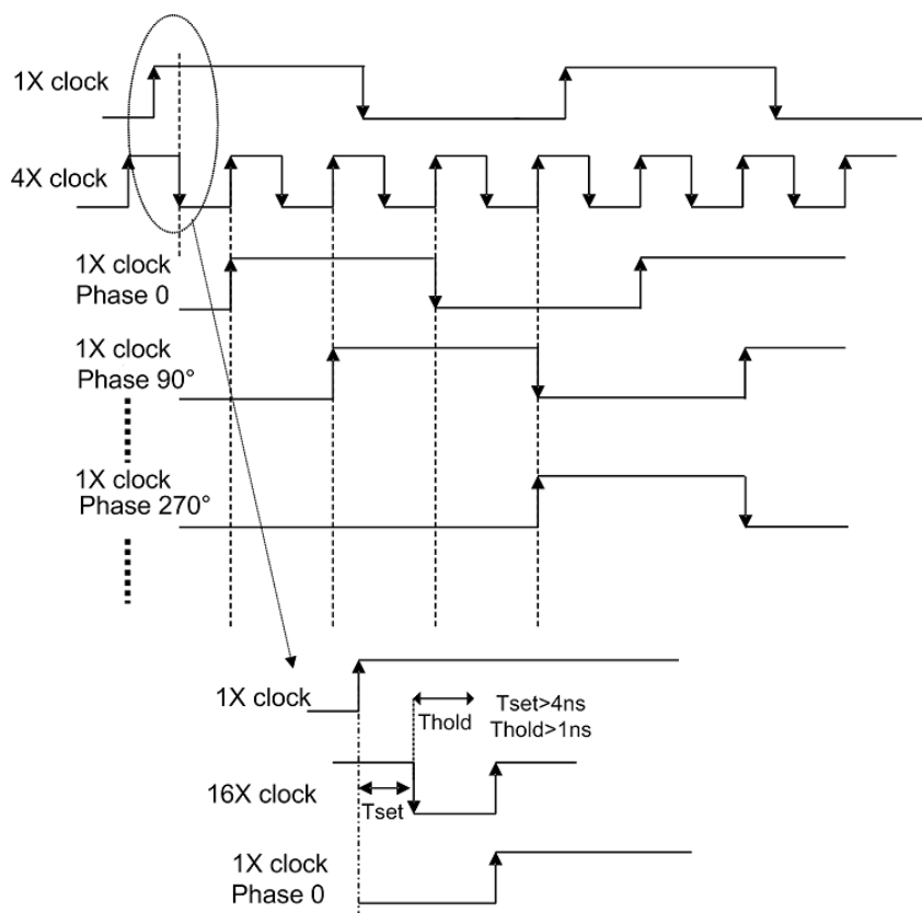
Figure 72. 8 \times f_{cw} and 4 \times f_{cw} Timing Diagram
