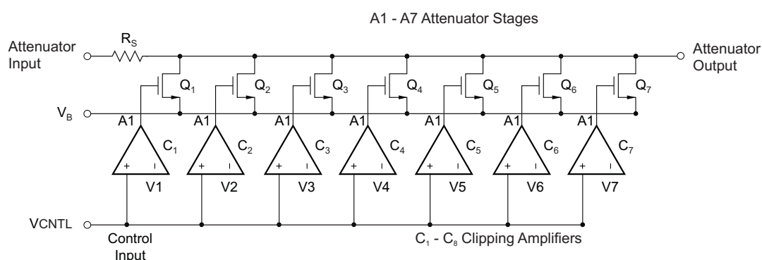
Figure 63. Simplified Voltage-Controlled Attenuator (Analog Structure)
