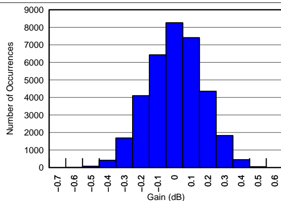
Figure 5. Gain Matching Histogram, V_{CNTL} = 0.6 V (34951 Channels)
