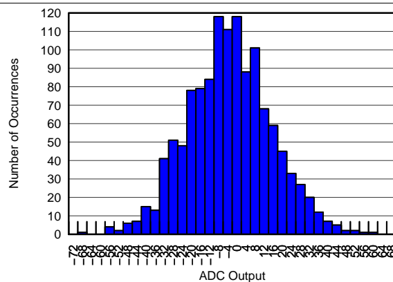
Figure 7. Output Offset Histogram, V_{CNTL} = 0 V (1247 Channels)
