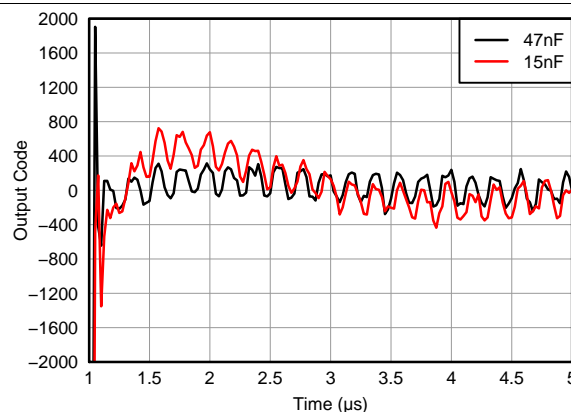
Figure 57. Overload Recovery Response vs INM Capacitor (Zoomed), V IN = 50 mVpp/100 μVpp, Max Gain
