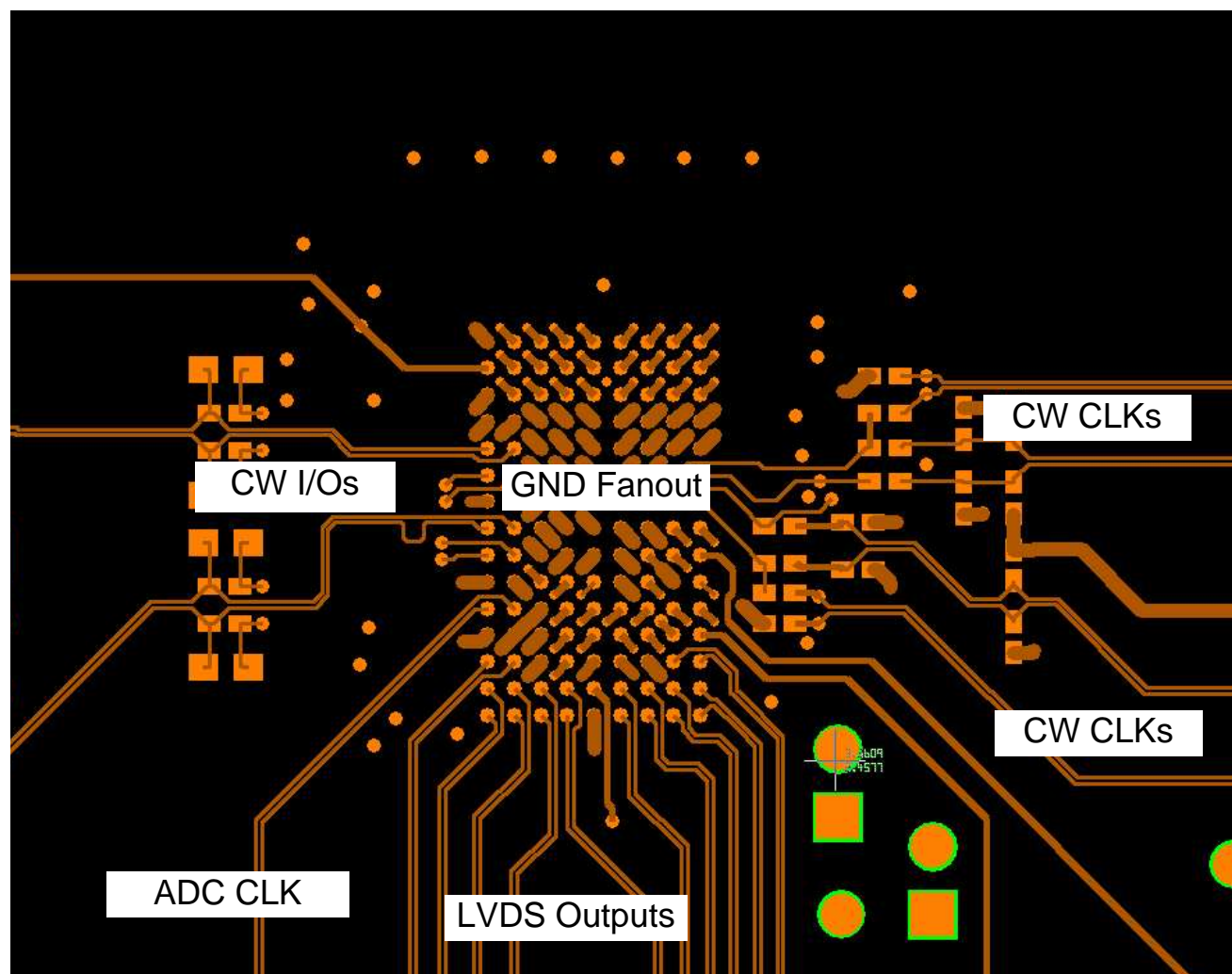
Figure 117. Layout Example
