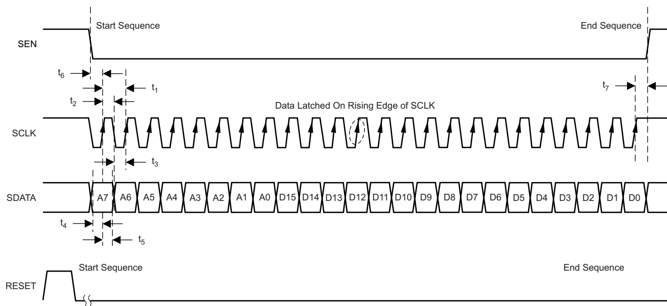
Figure 83. SPI Timing
