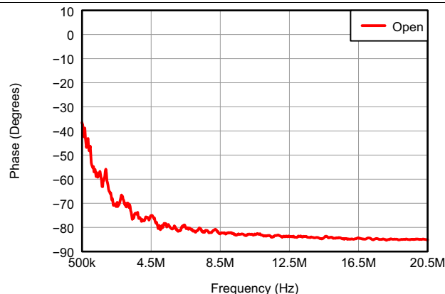
Figure 9. Input Impedance Without Active Termination (Phase)
