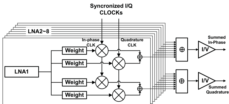
Figure 73. Block Diagram of 1 \times f_{CW} mode
