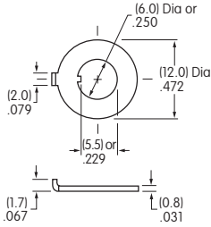
AT506M Locking Ring Steel with Zinc/Chromate
