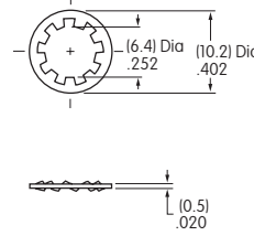
AT508 Lockwasher Steel with Zinc/Chromate (not supplied with splashproof models)
