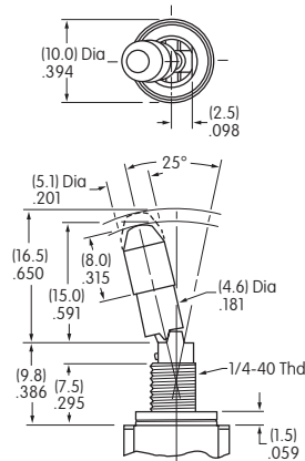
LL3 1/4-40 .295" (7.5mm) Threaded Splashproof with D Flat
