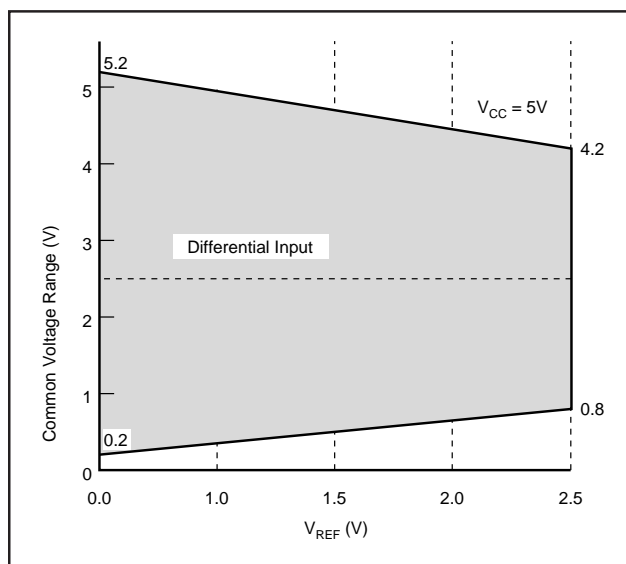
FIGURE 4. Differential Input—Common Voltage Range vs V_{REF} .
