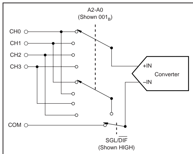
FIGURE 5. Simplified Diagram of the Analog Input.
