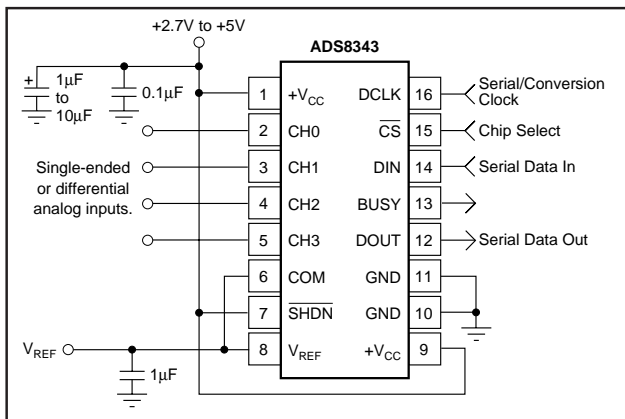
FIGURE 1. Basic Operation of the ADS8343.
