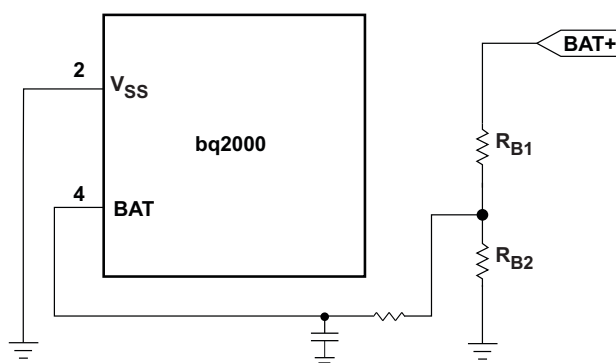
Figure 3. Battery Voltage Divider and Filter
