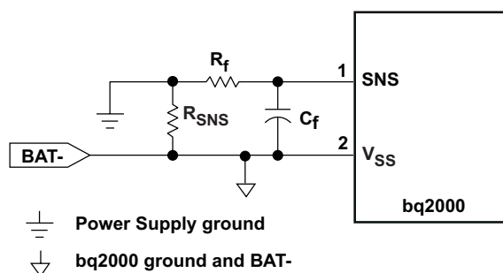
Figure 9. Current-Sensing Circuit
