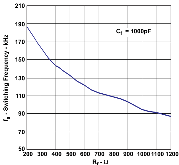
Figure 11. Switching Frequency vs Resistance
