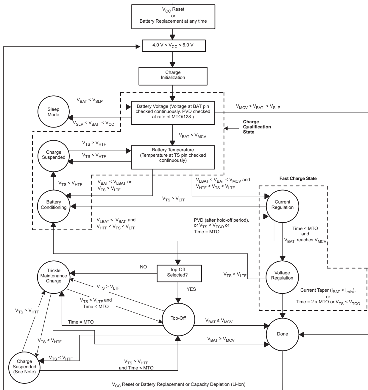
Figure 2. State Diagram
