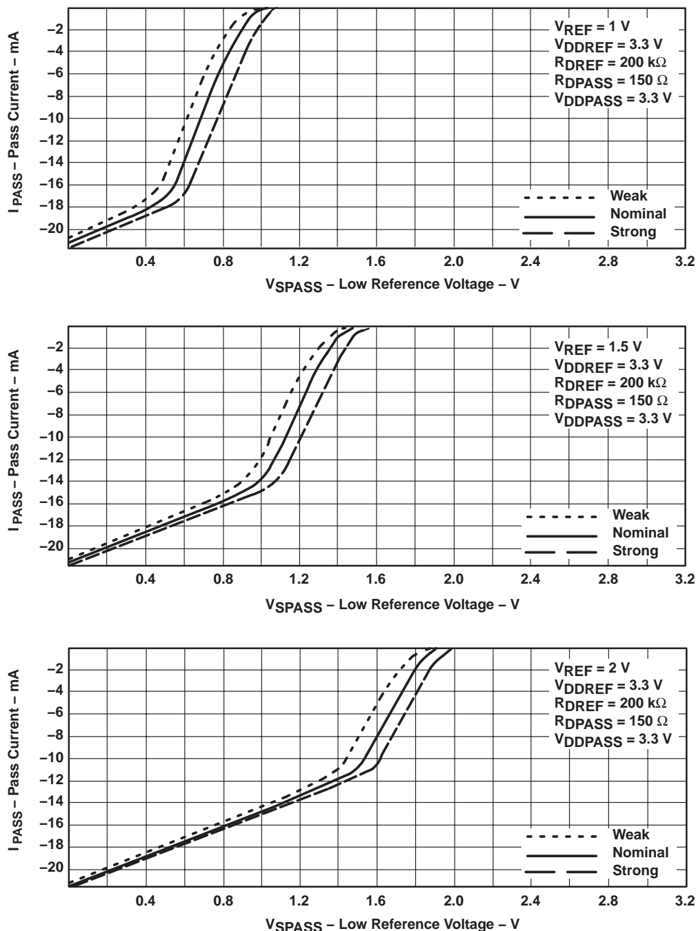
Figure 5. V-I Electrical Characteristics at Low V_{REF} Voltages
