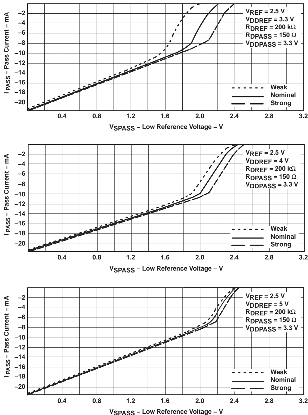
Figure 6. V-I Electrical Characteristics at V_{REF} = 2.5\text{ V}
